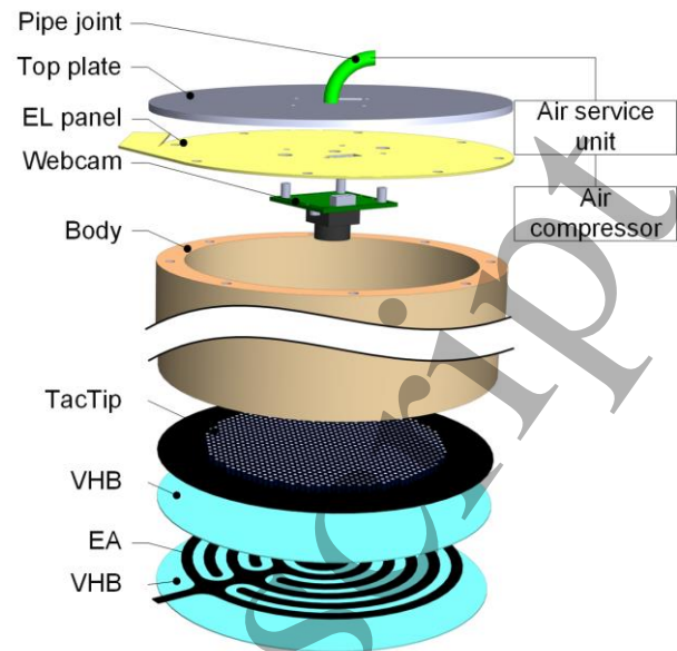
Figure 2. 3D schematic diagram of the soft-smart TacEA end effector.
