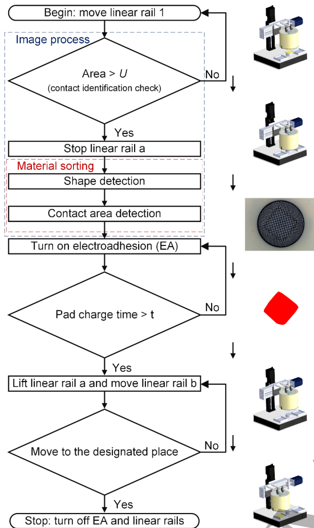
Figure 8. The movement and control flow chart of the TacEA material handling system.
