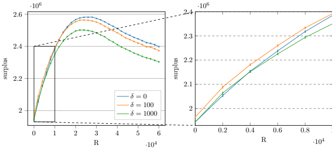
(a) Total surplus, S , for three different values of \delta . Central CDA are equivalent to \delta = 0 . For the replication results (Fig. 3), R = 2000 ; at this value (right, zoomed region), S_{\delta=100} > S_{\delta=1000} > S_{\delta=0} .
