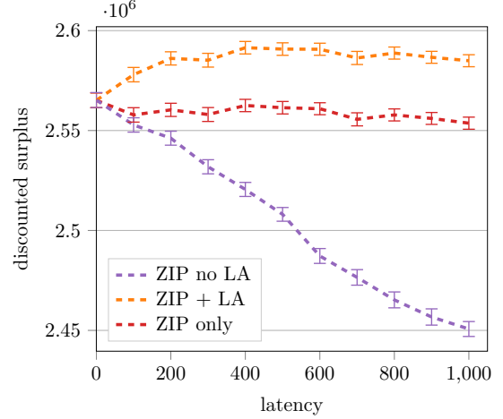
Fig. 6: Surplus for ZIP markets. S_{\text{CDA}}^{\text{ZIP}} \approx 2.57 \times 10^6 .
