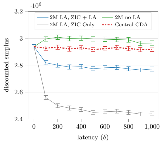
Fig. 3: Replication validation. Total discounted surplus, S , against \delta in 2M model, with/without LA, and a central CDA.
