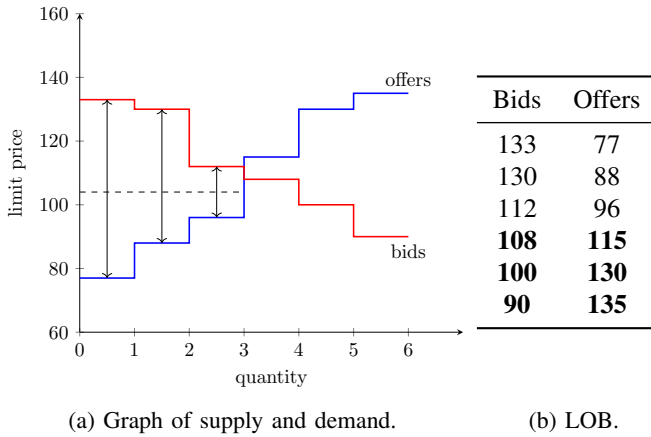
Fig. 1: Clearing operation in a DCA: (a) vertical arrows indicate orders matched at uniform clearing price, 104 (horizontal dashed line); (b) post-clearing, bold orders remain in the LOB.
