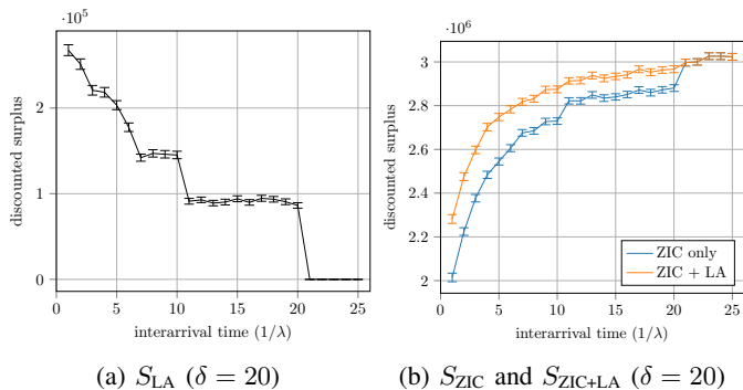
Fig. 4: Discounted surplus, S , against interarrival time of traders, 1/\lambda . LA profits are eliminated when 1/\lambda > \delta = 20 .
