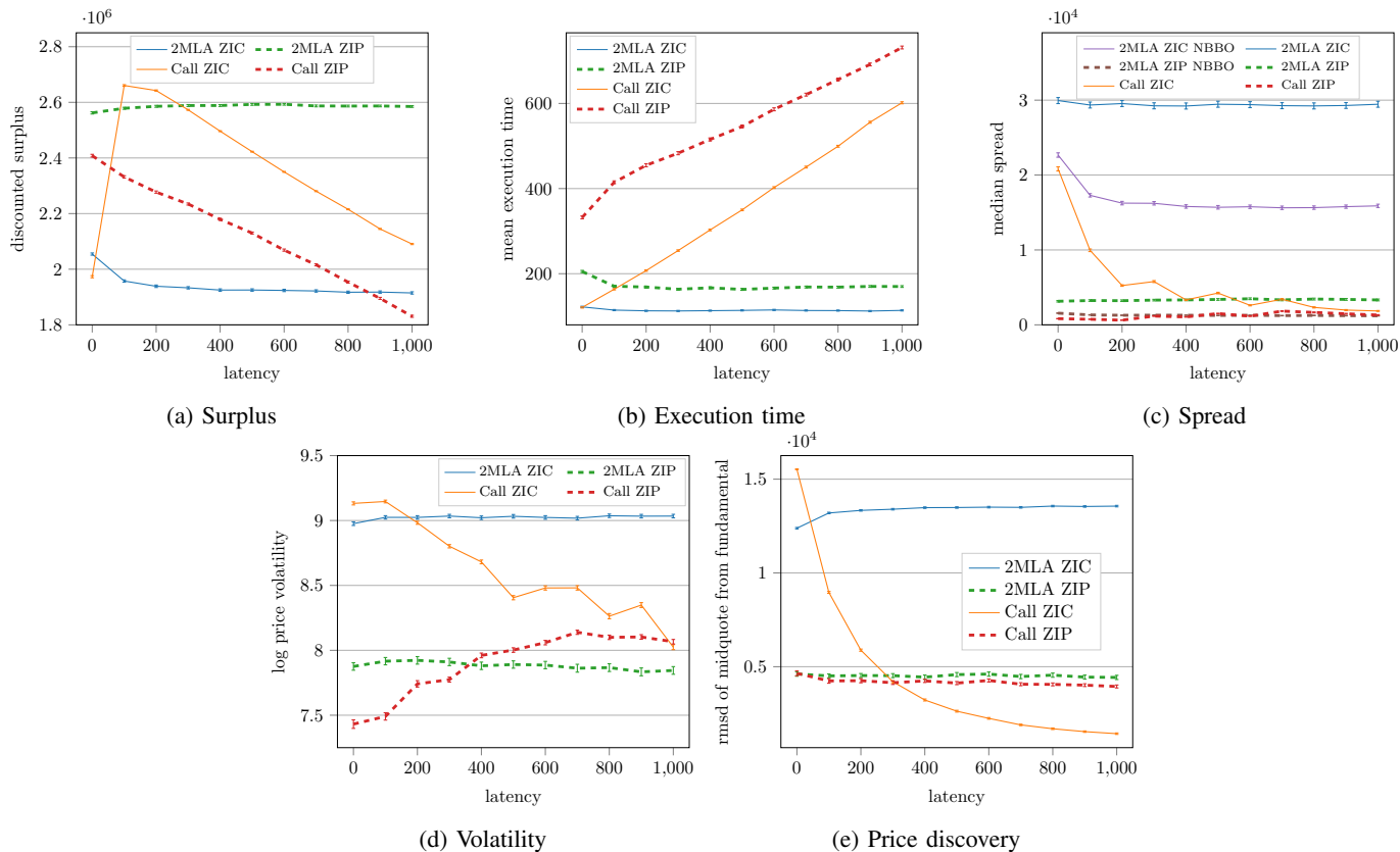
Fig. 7: Comparison between CDA and call auction (DCA), for models containing ZIC (solid line) and ZIP (dashed) traders.
