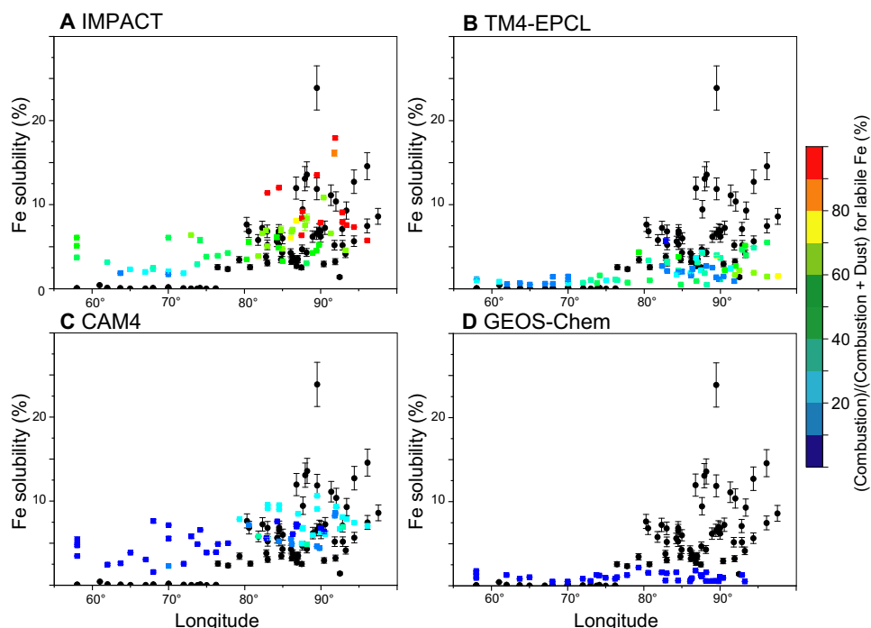
Fig. 2. Comparison of simulated atmospheric Fe solubility with field data (black circles) over the Bay of Bengal and Arabian Sea. (A to D) The color represents the simulated (combustion)/(combustion + dust) ratio (percent) for labile Fe concentration in aerosols.
