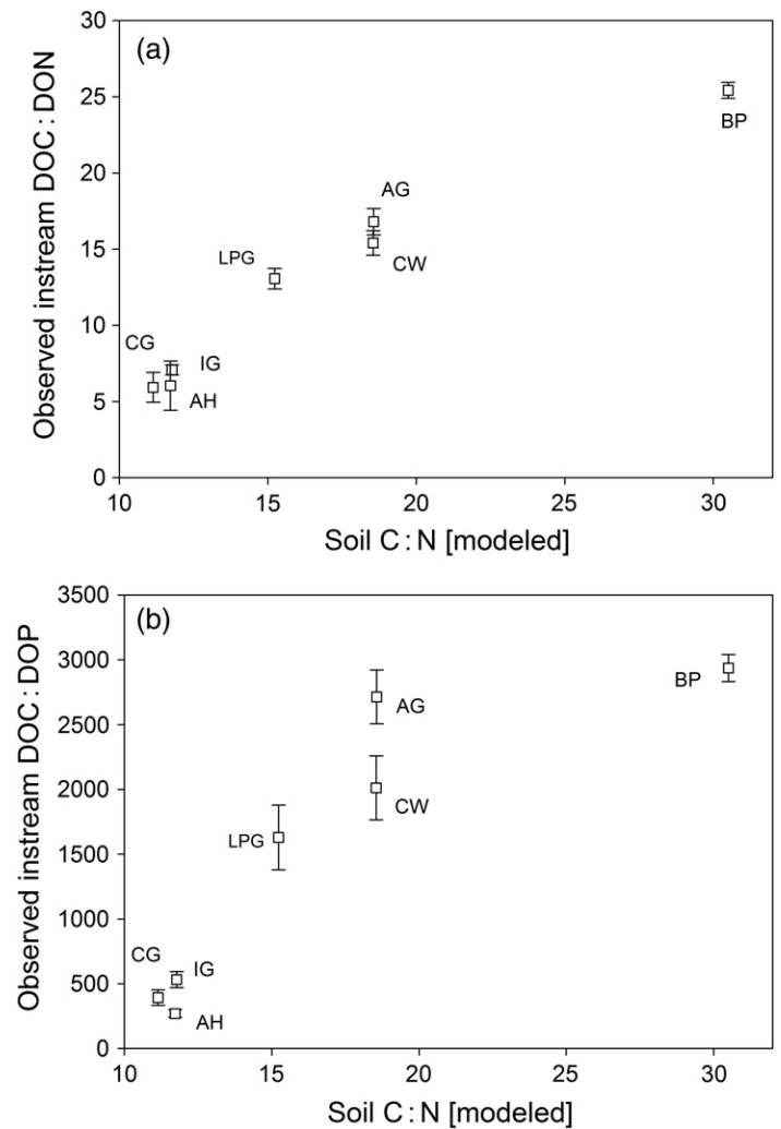
Fig. 5. Modeled soil C : N ratio vs. (a) observed instream DOC : DON and (b) observed instream DOC : DOP grouped by land cover classification. Data are mean values for both modeled and observed data \pm SEM grouped by dominant land cover classification (defined as a single land cover classification accounting for > 50% of catchment area).
