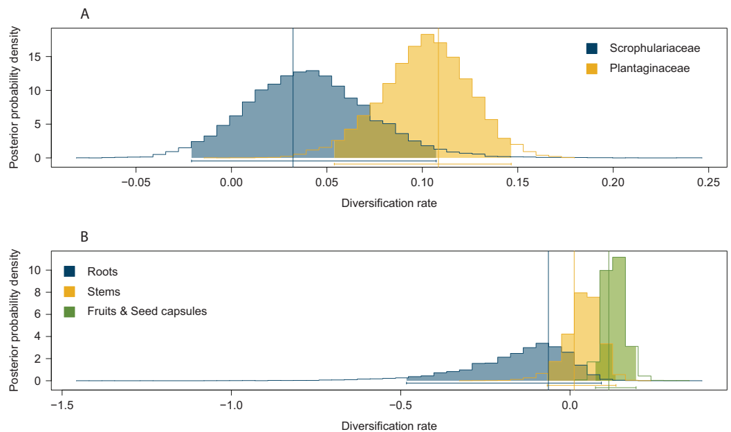
Figure 4 Posterior probability density plots of net diversification rates ( \lambda-\mu ) for Rhinusa and Gymnetron weevils associated with two traits of host plant use. (A) Use of two different plant families as hosts, (B) parasitic behavior on three different plant organs. Parameters were estimated from the MCC tree generated with BEAST under BiSSE and MuSSE models, respectively. Vertical lines represent mean maximum likelihood estimates from 1,000 post burn-in trees inferred with BEAST.
