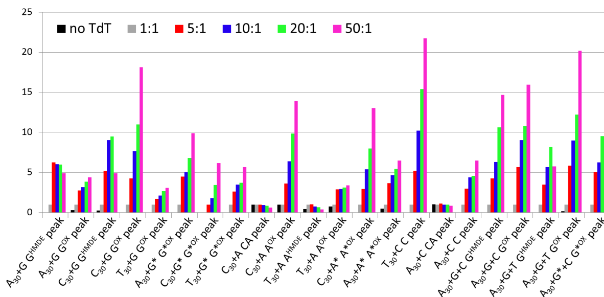
Figure 6. Normalized intensities of the respective peaks gained for all combinations of primers and dNTPs used for the TdT tailing reaction, including combinations with two mixed dNTPs (A 30 +G+C, A 30 +G+T and A 30 +G*+C).
