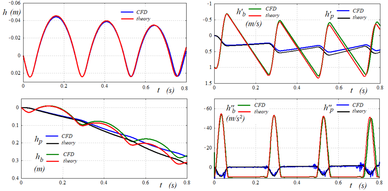
Figure 5: Comparison of the theoretical and numerical results for the plate indentation h , displacements h_p and h_b , speeds h'_p and h'_b and the accelerations h''_p and h''_b of the plate and the body, respectively, as functions of time t .
