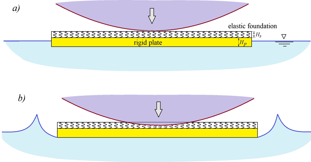
Figure 4: Impact on a floating plate with an elastic layer on the top of it before the interaction (a) and during the interaction (b).
