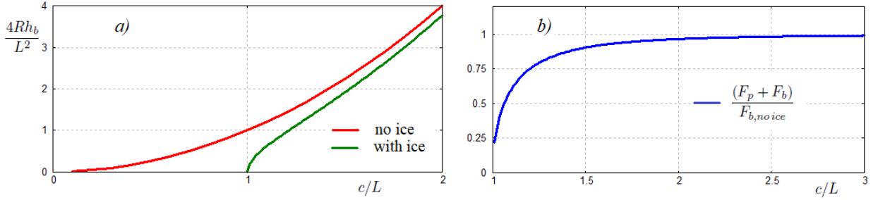
Figure 7: Non-dimensional penetration depth of the body (a) and the non-dimensional hydrodynamic force (b) as functions of the scaled length, c/l , of the wetted part of the body surface.
