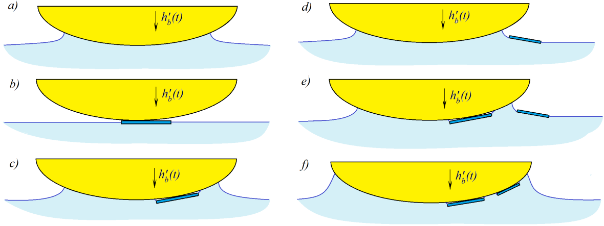
Figure 1: Two-dimensional slamming for open water (a), with ice floe (b), which is attached to the body surface later on (c), with an ice floe near the impact region (d), several floes under and near the body surface (e) and floes on the body surface (f).
