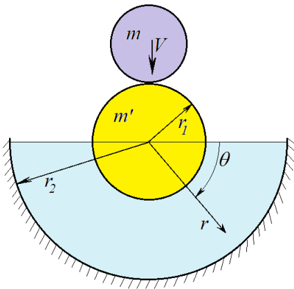
Figure 3: Impact of two spheres studied by Joukowski (1884).
