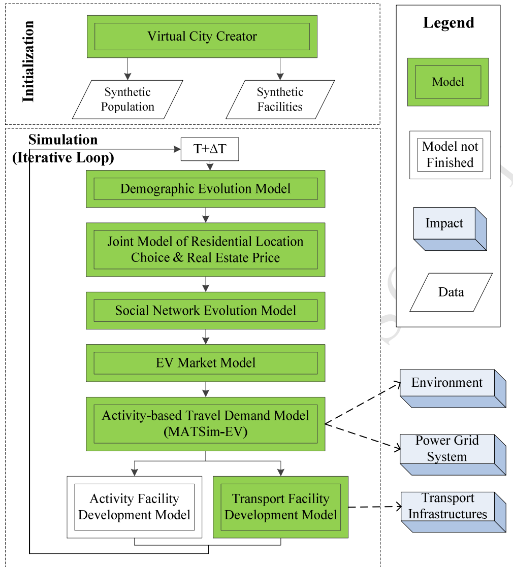
Figure 1 Framework of the SelfSim-EV Model (Zhuge and Shao, 2018a; Zhuge and Shao, 2018b; Zhuge et al., 2018a)
