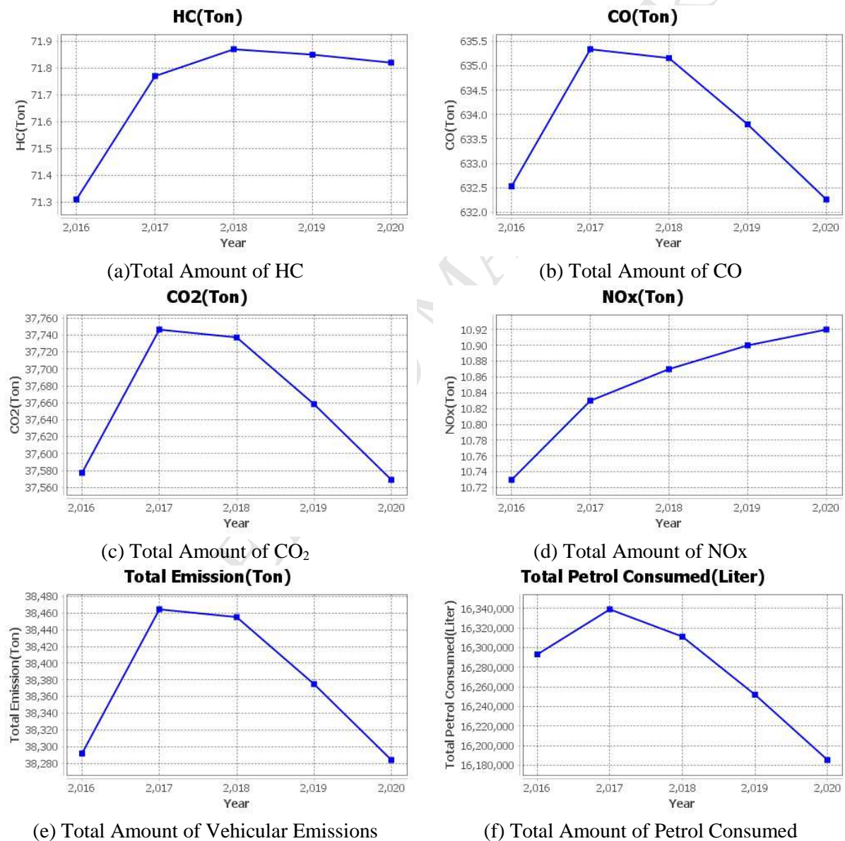
Figure 11 Amounts of Petrol Consumed and Vehicular Emissions in One Particular Weekday from 2016 to 2020
