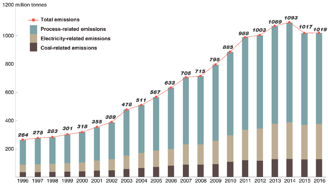
Figure 2 CO 2 emissions from China's cement industry
