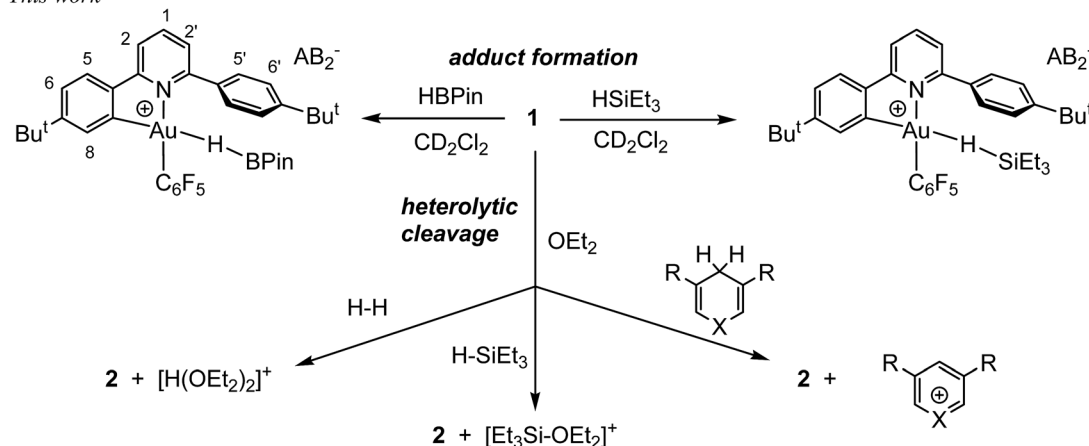
Scheme 1 Reaction outlines including the atom labelling scheme used in NMR assignments.
