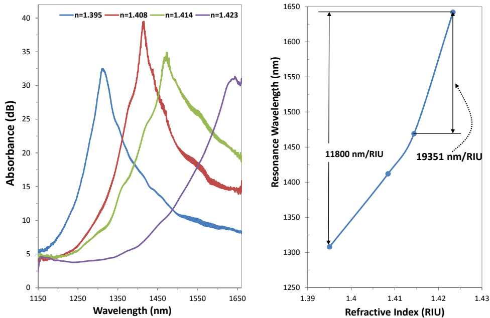
Fig. 4. (Left) Spectral response of a LMR optical fiber refractometer based on ITO thin film when the external refractive index changes from 1.395 to 1.423; (Right) Spectral position of the LMR band versus external refractive index.
