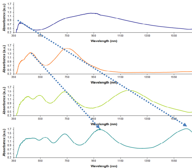
Fig. 3. Optical spectra of a LMR optical fiber device when the thickness of the supporting layer is increased. In this case, the supporting layer was a Layer-by-Layer assembled coating of [TiO 2 /PSS], and the number of bilayers from top to bottom was 10, 30, 50 and 70. Details about the fabrication process of these coatings can be found in [9]
