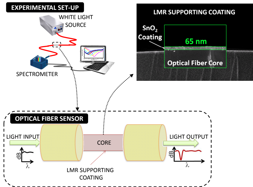
Fig. 2. Top-left, the simplified experimental set-up to observe LMRs in optical fiber; bottom, the optical fiber sensor based on LMR and top-right, SEM images of a LMR supporting layer.
