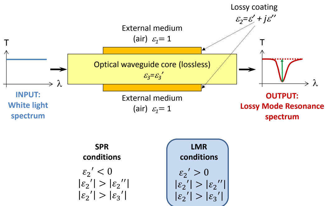
Fig. 1. Schematic of the waveguide coated with a thin film of an optical absorbing material that fulfills the conditions to generate LMRs
