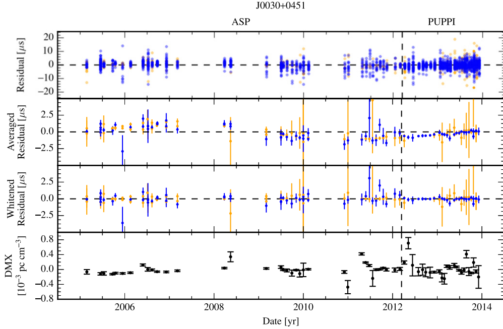
Figure 8. Timing summary for PSR J0030+0451. Colors are blue: 1.4 GHz, purple: 2.3 GHz, green: 820 MHz, orange: 430 MHz, red: 327 MHz. In the top panel, individual points are semi-transparent; darker regions arise from the overlap of many points.
