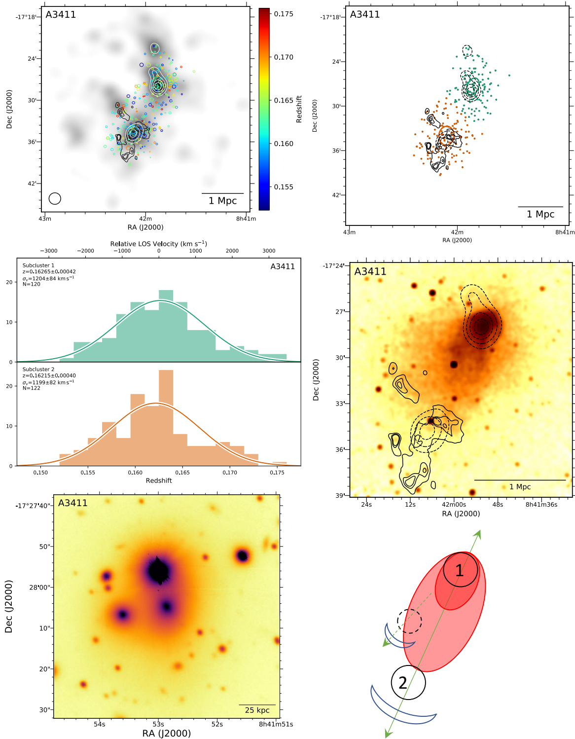
Figure 26. Abell 3411 Top left: DS-test over red sequence Subaru/SuprimeCam r-band luminosity distribution with linearly spaced white contours. The black contours show GMRT 325 MHz contours (van Weeren et al. 2017). Top right: Subcluster membership of spectroscopic cluster members assigned with our GMM analysis. The same GMRT contours (solid) and red sequence luminosity contours (dashed) are depicted. Middle left: Subcluster redshift histogram with colors matching the image at the top right. Middle right: 215 ks Chandra image with the same GMRT radio contours (solid) and red sequence luminosity contours (dashed). Bottom left: 150 kpc cutout of the Subaru r-band image centered on the cluster BCG in subcluster 1. Bottom right: Preferred merger scenario. A3411 is composed of at least two subclusters, where the northern subcluster 1 is A3411 and the southern 2 is A3412. Subcluster 1 is associated with a cool-core remnant and wake feature indicating the ICM is traveling northward. The two subclusters have very similar velocity dispersions and redshifts suggesting a 1:1 mass ratio merger in the plane of the sky. There is evidence of composite structure in subcluster 2 as presented in van Weeren et al. (2017), where a small subcluster has created a shock that reaccelerated particles associated with an AGN.
