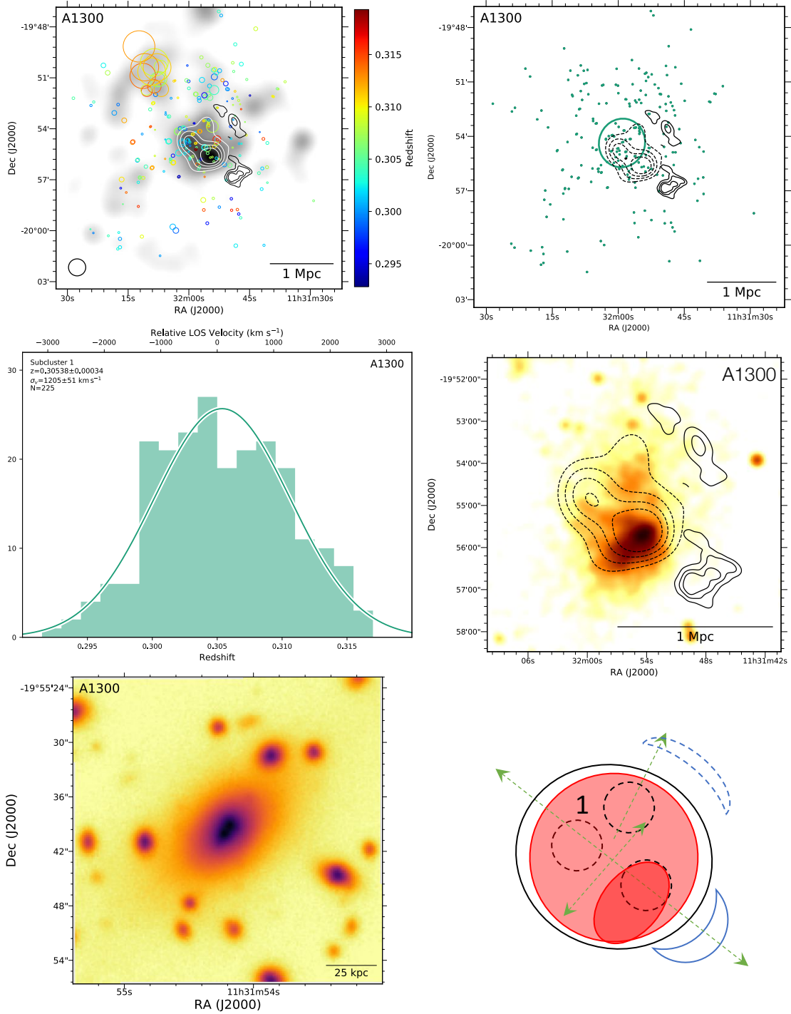
Figure 16. Abell 1300 Top left: DS-test over red sequence r-band luminosity distribution with linearly space white contours. The black contours show the 325 MHz GMRT contours (Venturi et al. 2013). Top right: Subcluster membership of spectroscopic cluster members assigned with our GMM analysis. The same GMRT contours (solid) and red sequence luminosity contours (dashed) are depicted. The small projected separation and low spectroscopic survey density likely contributes to a single halo model being preferred by the BIC analysis. Middle left: Subcluster redshift histograms with colors matching the image at the top right. Middle right: 100 ks Chandra image with the same GMRT radio contours (solid) and red sequence luminosity contours (dashed). The relics and disturbed ICM are suggestive of a complex merger between at least three subclusters. Bottom left: 150 kpc cutout of the Subaru/SuprimeCam r-band image centered on the cluster BCG. Bottom right: Proposed merger scenario. A1300 is a difficult to interpret merger with likely at least three subclusters. The X-ray surface brightness morphology is suggestive of of an additional merger axis associated with the an additional merger in the southwest to northeast direction. The BCG is elongated along the same axis. Inspection of the higher resolution HST RELICS images at https://www.spacetelescope.org/images/potw1745a/ show the BCG is actually composed of two luminosity peaks along this axis.
