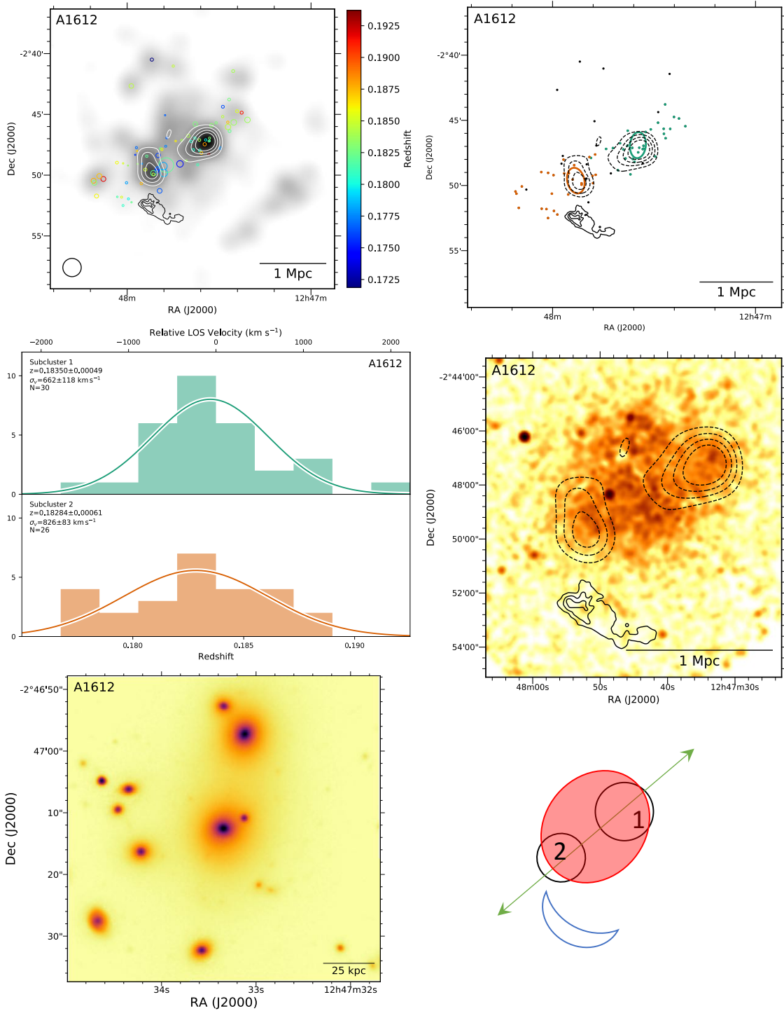
Figure 17. Abell 1612 Top left: DS-test over red sequence r-band luminosity distribution with linearly space white contours. The black contours show the 325 MHz GMRT contours (van Weeren et al. 2011b). Top right: Subcluster membership of spectroscopic cluster members assigned with our GMM analysis. The same GMRT contours (solid) and red sequence luminosity contours (dashed) are depicted. Middle left: Subcluster redshift histograms with colors matching the image at the top right. Middle right: 100 ks Chandra image with the same GMRT radio contours (solid) and red sequence luminosity contours (dashed). The relics and disturbed ICM are suggestive of a complex merger between at least three subclusters. Bottom left: 150 kpc cutout of the Subaru/SuprimeCam r-band image centered on the cluster BCG. Bottom right: Proposed merger scenario. The radio relic location perhaps suggests an off axis merger; however, inspection of the 610 MHz GMRT in Figure 2 of van Weeren et al. (2011b) suggests the relic is closely linked to the AGN of the BCG suggesting the shock may be larger than the radio relic, but the weak shock is only accelerating the electrons where they were pre-accelerated by the AGN (e.g., van Weeren et al. 2017).
