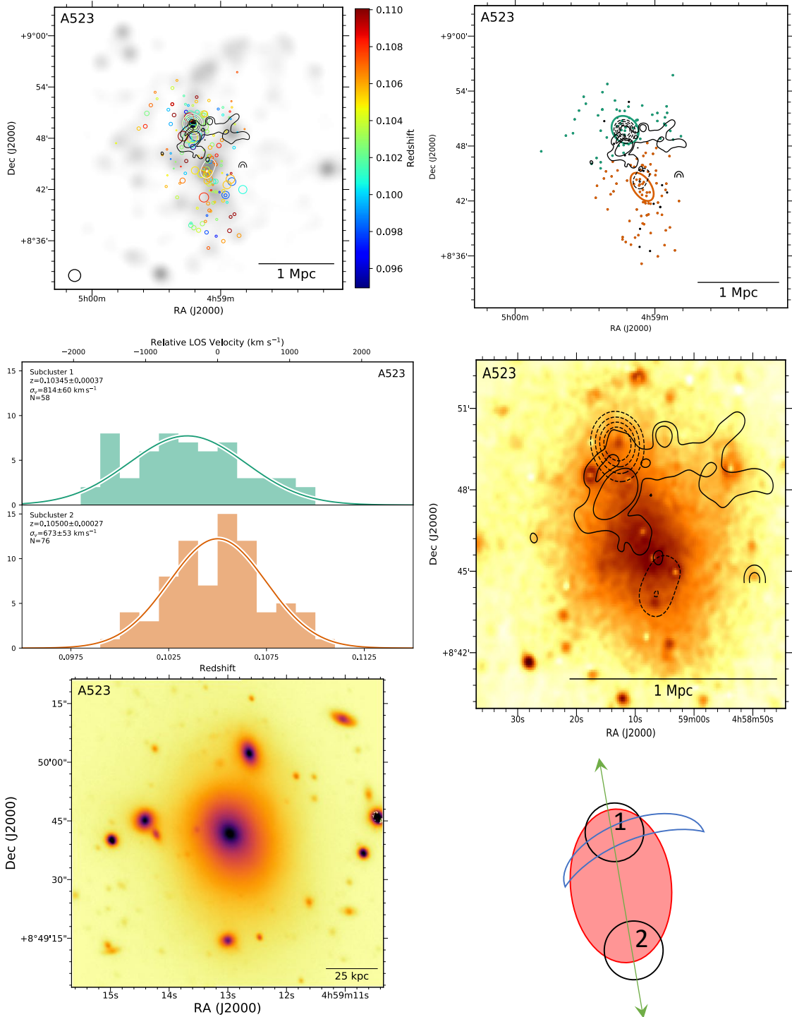
Figure 12. Abell 523 Top left: DS-test over red sequence r-band luminosity distribution with linearly spaced white contours. The black contours show the 1.4 GHz VLA contours (van Weeren et al. 2011b). Top right: Subcluster membership of spectroscopic cluster members assigned with our GMM analysis. The same VLA contours (solid) and red sequence luminosity contours (dashed) are depicted. Middle left: Subcluster redshift histograms with colors matching the image at the top right. Middle right: 30 ks Chandra image with the same VLA radio contours (solid) and red sequence luminosity contours (dashed). A bimodal merger scenario is evident, but the radio emission is not clearly tracing a potential merger induced shock between subclusters 1 and 2. Bottom left: 150 kpc cutout of the Subaru/SuprimeCam r-band image centered on the BCG of subcluster 1. Bottom right: Proposed merger scenario. A523 is a clean bimodal merger with a difficult to interpret radio feature that has been debated in the literature.
