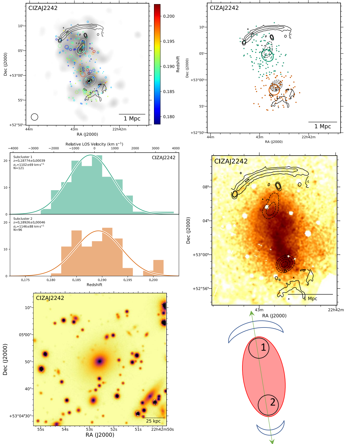
Figure 27. CIZA J2242.8+5301 Top left: DS-test over red sequence Subaru/SuprimeCam i-band luminosity distribution with linearly space white contours. The black contours show WSRT 1382 MHz contours (van Weeren et al. 2010). Top right: Subcluster membership of spectroscopic cluster members assigned with our GMM analysis. The same WSRT contours (solid) and red sequence luminosity contours (dashed) are depicted. Middle left: Subcluster redshift histogram with colors matching the image at the top right. Middle right: 206 ks Chandra image with the same WSRT radio contours (solid) and red sequence luminosity contours (dashed). Bottom left: 150 kpc cutout of the Subaru i-band image centered on the cluster BCG in subcluster 1. Bottom right: Preferred merger scenario. CIZA J2242 is composed of at least two subclusters with similar velocity dispersions and redshifts suggesting a 1:1 merger in the plane of the sky. The ICM has been extremely disrupted and is situated between the two subclusters. The famous ‘Sausage’ radio relic in the north has been studied across a wide range of frequencies, and dark matter-galaxy offsets have been detected in this cluster (Jee et al. 2016). The high mass, simple geometry, and extreme shock features have motivated a number of simulation studies as well.
