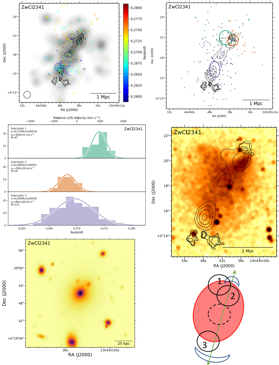
Figure 37. ZwCl 2341.1+0000 Top left: DS-test over red sequence Subaru/SuprimeCam r-band luminosity distribution with linearly spaced white contours. The black contours show GMRT 610 MHz contours (van Weeren et al. 2009b). Top right: Subcluster membership of spectroscopic cluster members assigned with our GMM analysis. The same WSRT contours (solid) and red sequence luminosity contours (dashed) are depicted. Middle left: Subcluster redshift histogram with colors matching the image at the top right. Middle right: 227 ks Chandra image with the same GMRT radio contours (solid) and red sequence luminosity contours (dashed). Bottom left: 150 kpc cutout of the Subaru r-band image centered on the cluster BCG in subcluster 1. Bottom right: Preferred merger scenario. We detect three subclusters with our GMM as well as a fourth that is evident in the red sequence luminosity distribution. Two subclusters (subclusters 2 and 3) and the candidate third situated in the middle of the cluster are aligned with the two radio relics. This suggests the dominant component of the merger is occurring along this axis with at least two subclusters partaking. Subcluster 1 is positioned to the east of subcluster 2, and is evident in both the X-ray surface brightness profile and red sequence luminosity. The disturbed gas suggests it has already merged, and the large line of sight velocity difference suggests line of sight motion.
