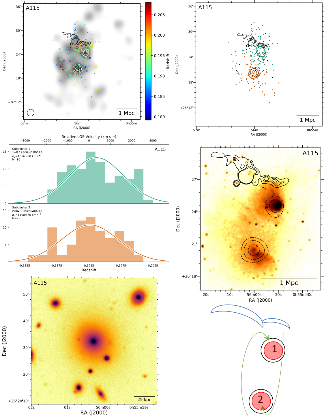
Figure 10. Abell 115 Top left: DS-test over red sequence i-band luminosity distribution with linearly space white contours. The black contours show the 1.4 GHz VLA contours (Govoni et al. 2001b). Top right: Subcluster membership of spectroscopic cluster members assigned with our GMM analysis. The same VLA contours (solid) and red sequence luminosity contours (dashed) are depicted. Middle left: Subcluster redshift histograms with colors matching the image at the top right. Middle right: 376 ks Chandra image with the same VLA radio contours (solid) and red sequence luminosity contours (dashed). The glancing merger scenario is clear from the swirling stream of X-ray emission. Bottom left: 150 kpc cutout of the Subaru/SuprimeCam image centered on the BCG of subcluster 2. Bottom right: Schematic of preferred merger scenario showing a large impact parameter merger and spiraling motion in the observed state.
