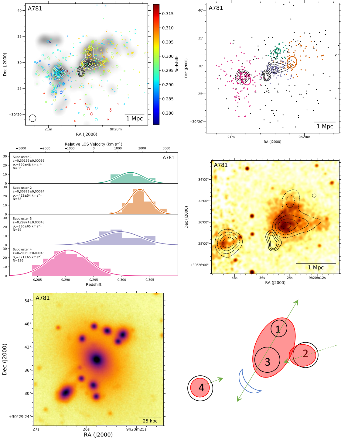
Figure 14. Abell 781 Top left: DS-test over red sequence i-band luminosity distribution with linearly space white contours. The black contours show the 325 MHz GMRT contours (Venturi et al. 2013). Top right: Subcluster membership of spectroscopic cluster members assigned with our GMM analysis. The same GMRT contours (solid) and red sequence luminosity contours (dashed) are depicted. Middle left: Subcluster redshift histograms with colors matching the image at the top right. Middle right: 48 ks Chandra image with the same WSRT radio contours (solid) and red sequence luminosity contours (dashed). The relic and disturbed ICM are suggestive of a merger between subclusters 1 and 3. Bottom left: 150 kpc cutout of the Subaru/SuprimeCam i-band image centered on the cluster BCG, which is associated with subcluster 3. Bottom right: Proposed merger scenario. The ICM is most disrupted between subclusters 1 and 3 with subcluster 2 having a less disturbed ICM coincident with its galactic light. Subcluster 4 has yet to interact, but it will coalesce with the other subclusters in the future.
