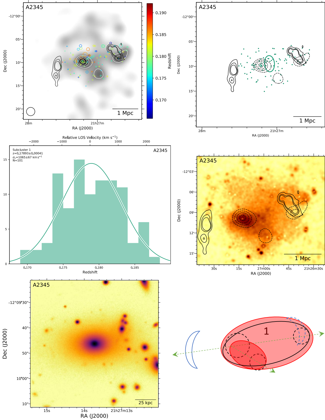
Figure 22. Abell 2345 Top left: DS-test over red sequence R-band luminosity distribution with linearly space white contours. The black contours show the 1.4 GHz VLA contours (Bonafede et al. 2009). Top right: Subcluster membership of spectroscopic cluster members assigned with our GMM analysis. The same VLA contours (solid) and red sequence luminosity contours (dashed) are depicted. The low spectroscopic survey density likely contributes to a single halo model being preferred. Middle left: Subcluster redshift histogram with colors matching the image at the top right. Middle right: 93 ks XMM image with the same VLA radio contours (solid) and red sequence luminosity contours (dashed). The relic at the northeast and the disturbed ICM are suggestive of a merger between at least three subclusters, perhaps with a large impact parameter for the northwest subcluster. Bottom left: 150 kpc cutout of the Subaru/SuprimeCam R-band image centered on the cluster BCG in the northeastern subcluster. Bottom right: Preferred merger scenario. The proximity of the western relic to the corresponding subcluster is difficult to explain in a scenario where the two relics were launched with the same merger.
