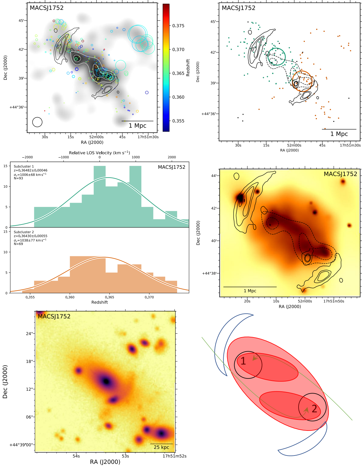
Figure 29. MACS J1752.0+4440 Top left: DS-test over red sequence Subaru/SuprimeCam i-band luminosity distribution with linearly spaced white contours. The black contours show WSRT 1.4 GHz contours (van Weeren et al. 2012a). Top right: Subcluster membership of spectroscopic cluster members assigned with our GMM analysis. The same WSRT contours (solid) and red sequence luminosity contours (dashed) are depicted. Middle left: Subcluster redshift histogram with colors matching the image at the top right. Middle right: 13 ks XMM image with the same WSRT radio contours (solid) and red sequence luminosity contours (dashed). Bottom left: 150 kpc cutout of the Subaru i-band image centered on the cluster BCG in subcluster 2. Bottom right: Preferred merger scenario. The X-ray image shows evidence for two ‘bullets’ that just missed and are beginning to orbit one another counter-clockwise. There two relics are bright and suggest a major merger despite not being head-on. The two subclusters have similar velocity dispersions and line of sight velocities suggesting the orbital plane is perpendicular to the line of sight.
