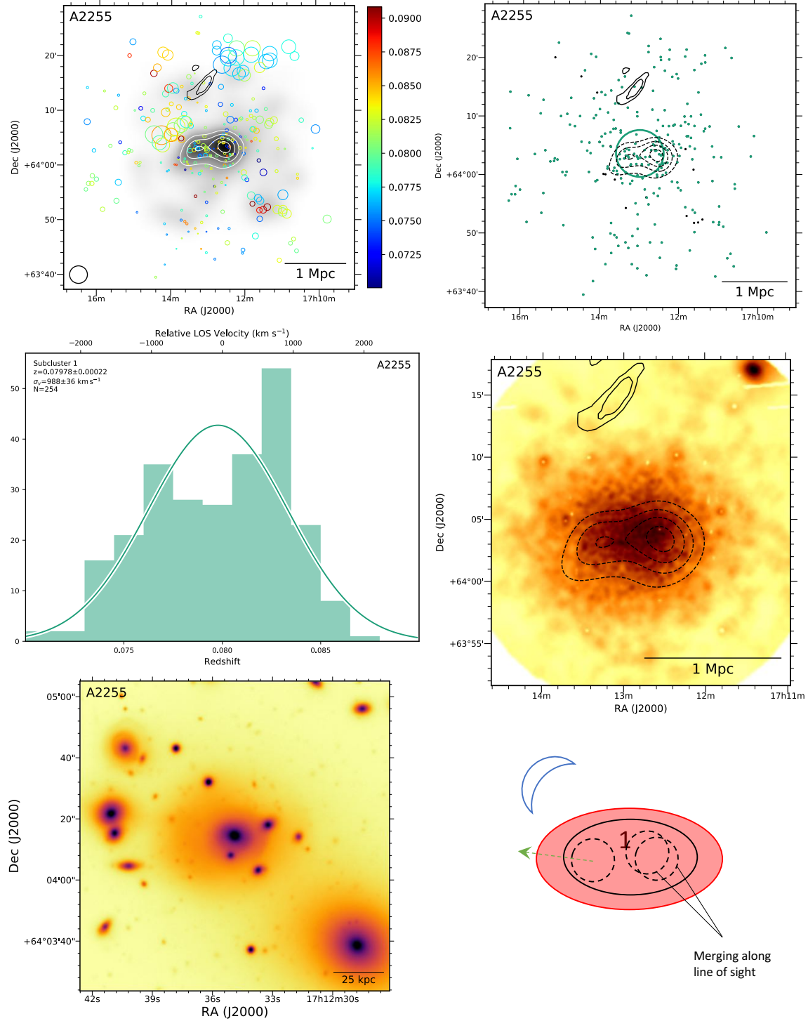
Figure 21. Abell 2255 Top left: DS-test over red sequence R-band luminosity distribution with linearly space white contours. The black contours show the 350 MHz WSRT contours (Pizzo & de Bruyn 2009). Top right: Subcluster membership of spectroscopic cluster members assigned with our GMM analysis. The same WSRT contours (solid) and red sequence luminosity contours (dashed) are depicted. The small projected separation and low spectroscopic survey density likely contributes to a single halo model being preferred. Middle left: Subcluster redshift histograms with colors matching the image at the top right. Middle right: 42 ks XMM image with the same WSRT radio contours (solid) and red sequence luminosity contours (dashed). The relic at the northeast and the disturbed ICM are suggestive of a merger between at least three subclusters. Bottom left: 150 kpc cutout of the Subaru/SuprimeCam R-band image centered on the cluster BCG in the western half of the cluster. The second BCG apparent in the image has a \sim 2000 km s -1 line of sight velocity difference, which is suggestive of a merger along the line of sight. Bottom right: Preferred merger scenario. The elongation of the X-ray surface brightness suggests a second plane of the sky merger component in addition to the line of sight merger. We do not make a prediction of which subclusters merged to launch the radio relic. We can not rule out further complications in this system.
