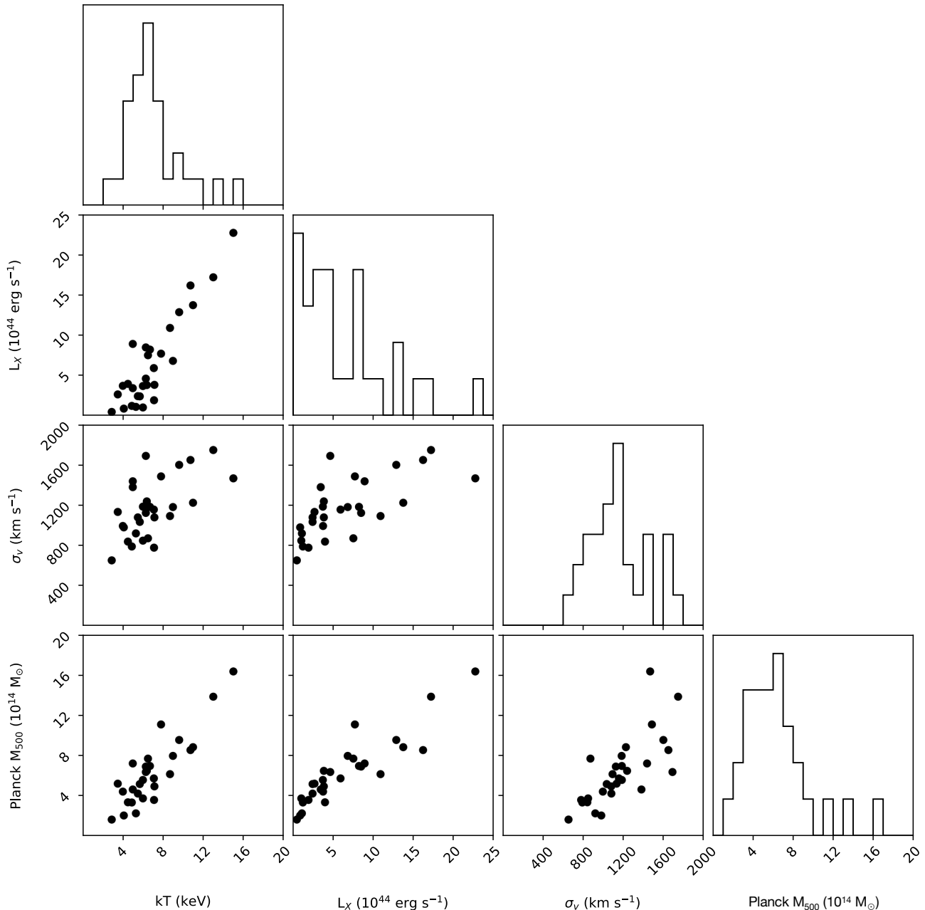
Figure 43. Relationships between four global measures for 29 merging clusters. The clear positive correlation between each suggests that, measuring these values gives a first order understanding of the mass of a merging system. Furthermore, with further lensing and dynamical study, we may understand why given systems have higher \sigma_v with respect to merger dynamics.
