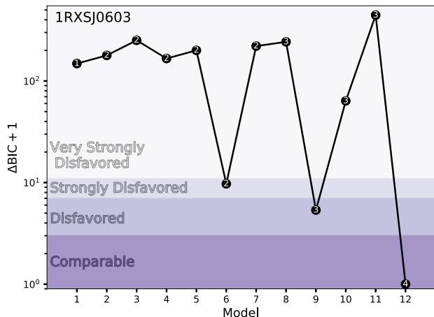
Figure 4. Bayesian Information Criterion scores relative to the most economical model for twelve 3D (RA, Dec, z) Gaussian Mixture Models fit to the 242 spectroscopic cluster member galaxies of 1RXSJ0603. The numbers in the black points indicate the number of subclusters included in a given model. The shaded regions roughly denote how a given model compares with the lowest BIC score (Kass & Raftery 1995). The most economical fit is a four component model (see Table 3 and 4). An analogous plot is not presented for each cluster; however, the \Delta\text{BIC} scores are presented in Table 4.
