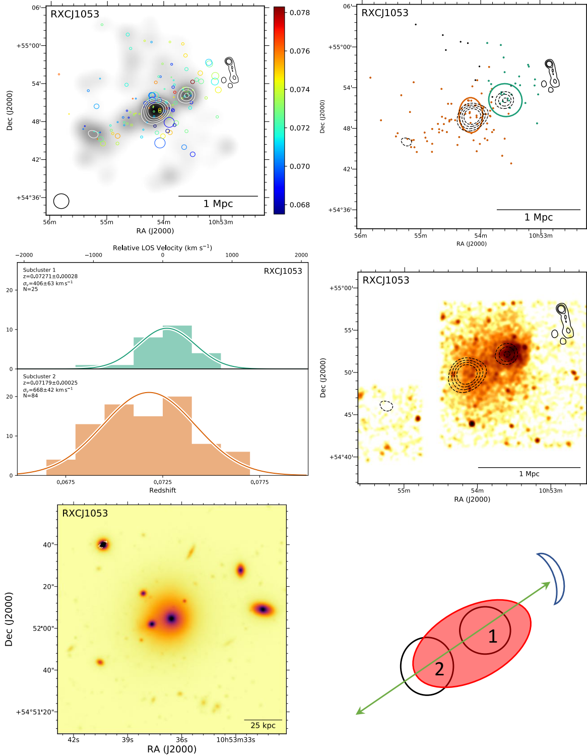
Figure 32. RXC J1053.7+5452 Top left: DS-test over red sequence Subaru/SuprimeCam r-band luminosity distribution with linearly spaced white contours. The black contours show WSRT 1382 MHz contours (Bonafede et al. 2014). Top right: Subcluster membership of spectroscopic cluster members assigned with our GMM analysis. The same WSRT radio contours (solid) and red sequence luminosity contours (dashed) are depicted. Middle left: Subcluster redshift histogram with colors matching the image at the top right. Middle right: 31 ks Chandra image with the same WSRT radio contours (solid) and red sequence luminosity contours (dashed). Bottom left: 150 kpc cutout of the Subaru r-band image centered on the cluster BCG in subcluster 1. Bottom right: Preferred merger scenario. The two subclusters and radio relic are aligned with the extended X-ray emission. Most of the mass appears to be associated with subcluster 2; however, the X-ray emission is associated with subcluster 1, which is perhaps a signature of a cool-core remnant. Deeper X-ray observations are necessary to reveal the nature of the ICM.
