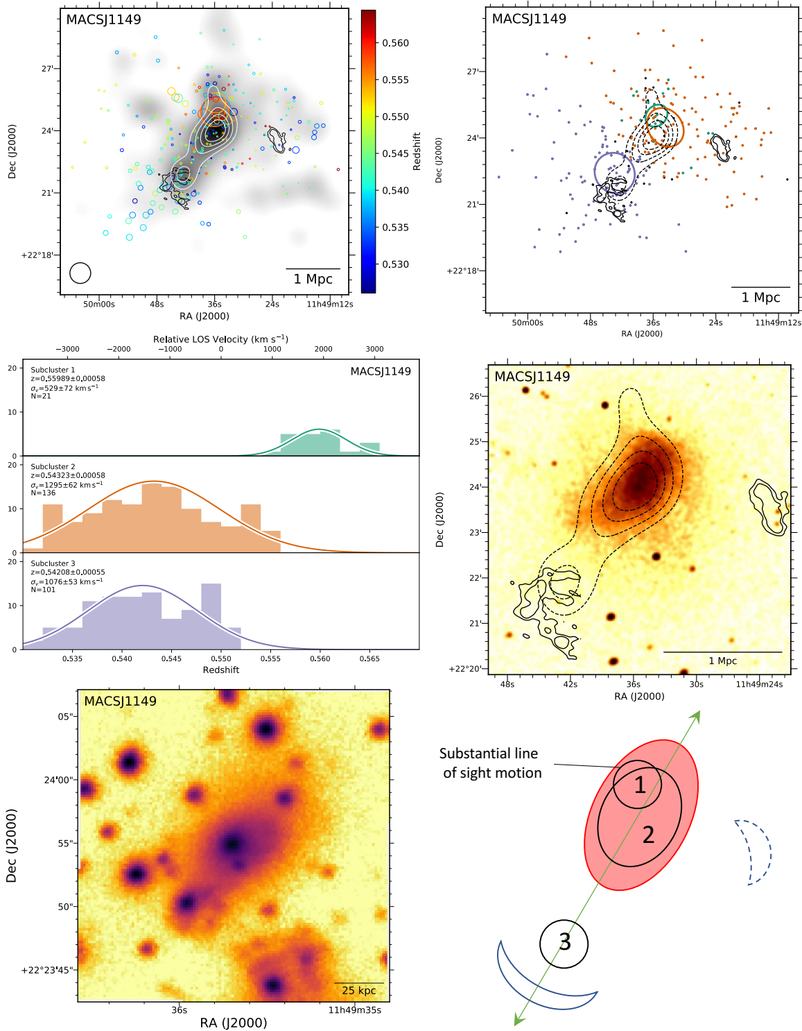
Figure 28. MACS J1149.5+2223 Top left: DS-test over red sequence Subaru/SuprimeCam R-band luminosity distribution with linearly spaced white contours. The black contours show GMRT 323 MHz contours (Bonafede et al. 2012). Top right: Subcluster membership of spectroscopic cluster members assigned with our GMM analysis. The same GMRT contours (solid) and red sequence luminosity contours (dashed) are depicted. Middle left: Subcluster redshift histogram with colors matching the image at the top right. Middle right: 372 ks Chandra image with the same GMRT radio contours (solid) and red sequence luminosity contours (dashed). Bottom left: 150 kpc cutout of the Subaru R-band image centered on the cluster BCG in subcluster 2. Bottom right: Preferred merger scenario. A detailed dynamical study of MACSJ1149 was presented in Golovich et al. (2016).
