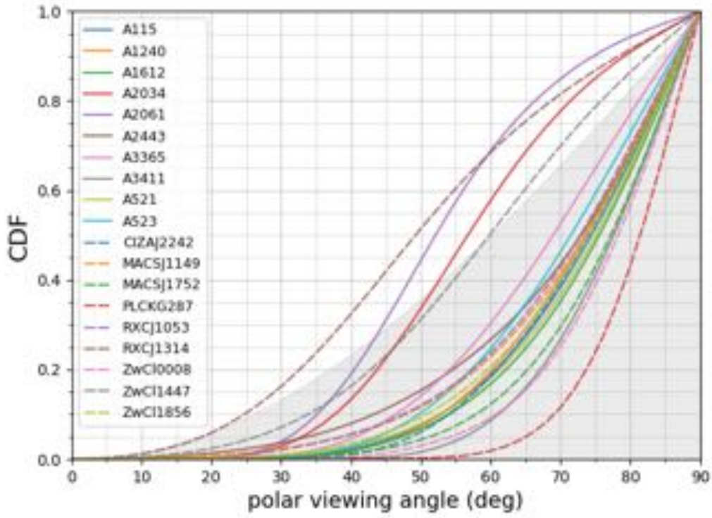
Figure 39. Cumulative distribution function for the polar viewing angle of 19 merging galaxy clusters in our sample. A merger in the plane of the sky is 90^\circ on this figure. The gray shaded boundary corresponds to expectation for random orientations. The median system has a 90% (50%) chance of being within 40^\circ ( 17^\circ ) of the plane of the sky.
