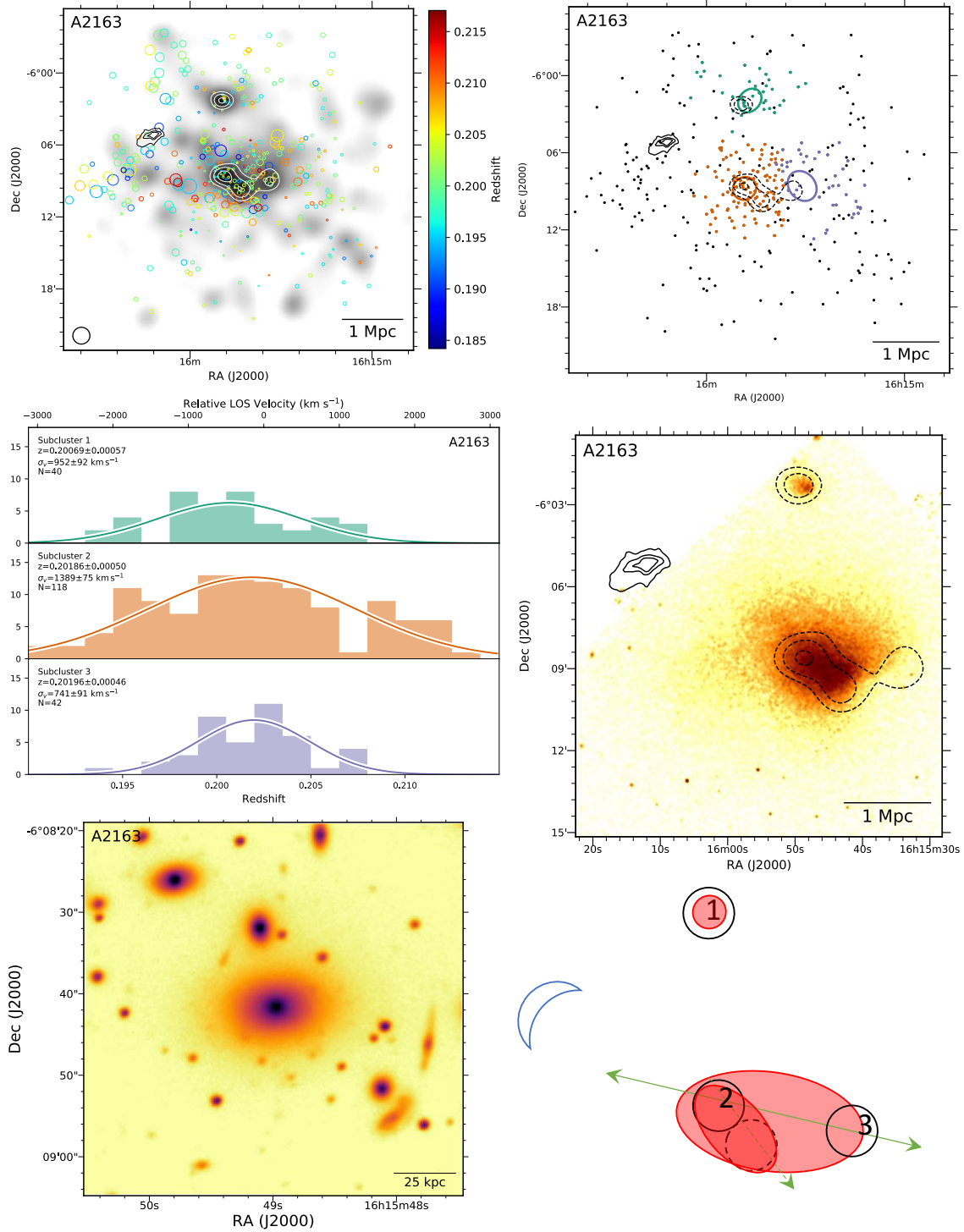
Figure 20. Abell 2163 Top left: DS-test over red sequence R-band luminosity distribution with linearly spaced white contours. The black contours show the 1.4 GHz VLA contours (Ferettil et al. 2001). Top right: Subcluster membership of spectroscopic cluster members assigned with our GMM analysis. The same VLA contours (solid) and red sequence luminosity contours (dashed) are depicted. The small projected separation between the two apparent subclusters comprising subcluster 2 likely contributes to a single halo describing this region. Middle left: Subcluster redshift histograms with colors matching the image at the top right. Middle right: 90 ks Chandra image with the same VLA radio contours (solid) and red sequence luminosity contours (dashed). The relic at the northeast and the disturbed ICM are suggestive of a merger between at least three subclusters. The northernmost subcluster 1 has yet to merge. Bottom left: 150 kpc cutout of the Subaru/SuprimeCam R-band image centered on the cluster BCG in subcluster 2. Bottom right: Preferred merger scenario. The large projected distance to the radio relic suggest an older merger. Subcluster 1 has yet to merge, and subcluster 3 has been stripped of its ICM suggesting it is post pericenter. A fourth subcluster is likely associated with the cool core remnant identified by Bourdin et al. (2011). This merger is very near core-crossing and likely contributing to the very high X-ray luminosity and SZ inferred mass.
