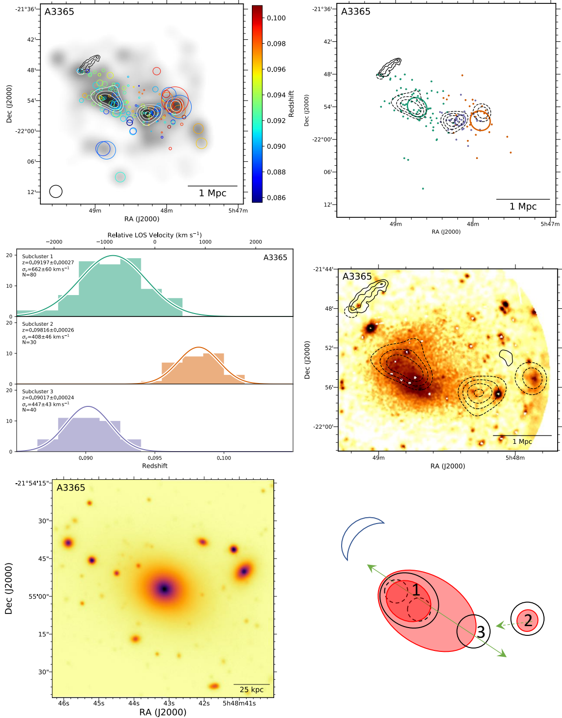
Figure 25. Abell 3365 Top left: DS-test over red sequence Subaru/SuprimeCam r-band luminosity distribution with linearly spaced contours. The black contours show the 1.4 GHz VLA contours (van Weeren et al. 2011b). Top right: Subcluster membership of spectroscopic cluster members assigned with our GMM analysis. The same VLA contours (solid) and red sequence luminosity contours (dashed) are depicted. Middle left: Subcluster redshift histogram with colors matching the image at the top right. Middle right: 161 ks XMM image with the same VLA radio contours (solid) and red sequence luminosity contours (dashed). Bottom left: 150 kpc cutout of the Subaru r-band image centered on the cluster BCG in subcluster 2. Bottom right: Preferred merger scenario. A3365 is composed of at least three subclusters with a merger occurring between subclusters 1 and 3 giving rise to the disturbed ICM and northeast relic. Subcluster 2 has a large line of sight velocity difference and undisturbed ICM suggesting it is still infalling with some component along the line of sight from the foreground, since it is redshifted relative to the rest of the cluster. There is evidence of composite structure in subcluster 1 which has two bright galaxies at either end of its associated red sequence luminosity peak as well as an elongated ridge of X-ray emission.
