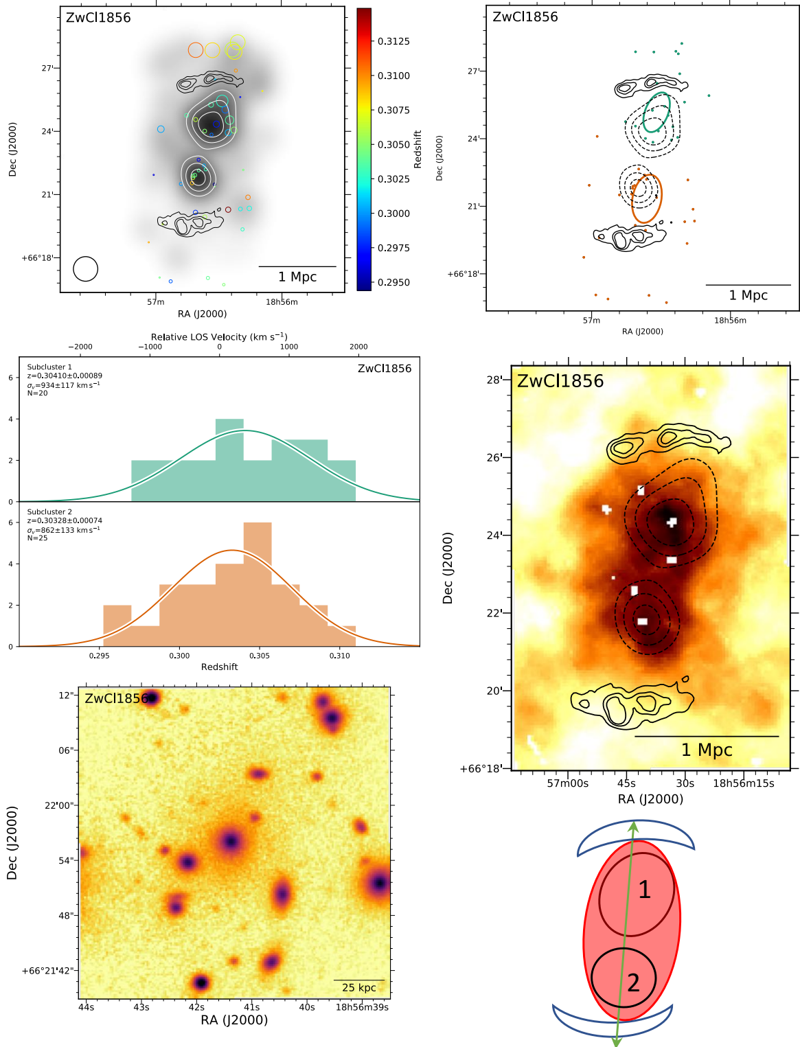
Figure 36. ZwCl 1856.8+6616 Top left: DS-test over red sequence Gemini/GMOS r-band luminosity distribution with linearly spaced white contours. The black contours show WSRT 1382 GHz contours (de Gasperin et al. 2014). Top right: Subcluster membership of spectroscopic cluster members assigned with our GMM analysis. The same WSRT contours (solid) and red sequence luminosity contours (dashed) are depicted. Middle left: Subcluster redshift histogram with colors matching the image at the top right. Middle right: 12 ks XMM image with the same WSRT radio contours (solid) and red sequence luminosity contours (dashed). Bottom left: 150 kpc cutout of the Gemini r-band image centered on the cluster BCG in subcluster 2. Bottom right: Preferred merger scenario. We detect two subclusters aligned with the X-ray surface brightness elongation and two radio relics suggesting a simple bimodal merger along a north-south axis. The two subclusters have similar velocity dispersions and redshifts; although, these are based on few galaxies per subcluster.
