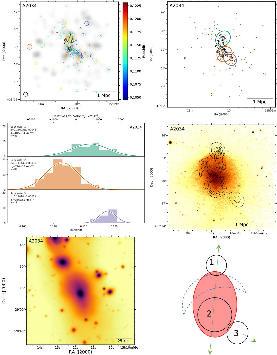
Figure 18. Abell 2034 Top left: DS-test over red sequence R-band luminosity distribution with linearly space white contours. The black contours show the 1.4 GHz WSRT contours (van Weeren et al. 2011b). Top right: Subcluster membership of spectroscopic cluster members assigned with our GMM analysis. The same WSRT contours (solid) and red sequence luminosity contours (dashed) are depicted. Middle left: Subcluster redshift histograms with colors matching the image at the top right. Middle right: 261 ks Chandra image with the same WSRT radio contours (solid) and red sequence luminosity contours (dashed). The relics and disturbed ICM are suggestive of a merger between at least two subclusters; however, the lack of X-ray emission with subcluster 3 suggests it was also involved. Bottom left: 150 kpc cutout of the Subaru/SuprimeCam R-band image centered on the cluster BCG in subcluster 2. Bottom right: Proposed merger scenario. A2034 is primarily a north to south merger with two complications. First, the shock has been classified as a cold front in the literature, which would better explain subcluster 1’s location; however, the relic candidate is coincident with this edge in the ICM. Second, subcluster 3 appears to have exited toward the southwest having its ICM stripped.
