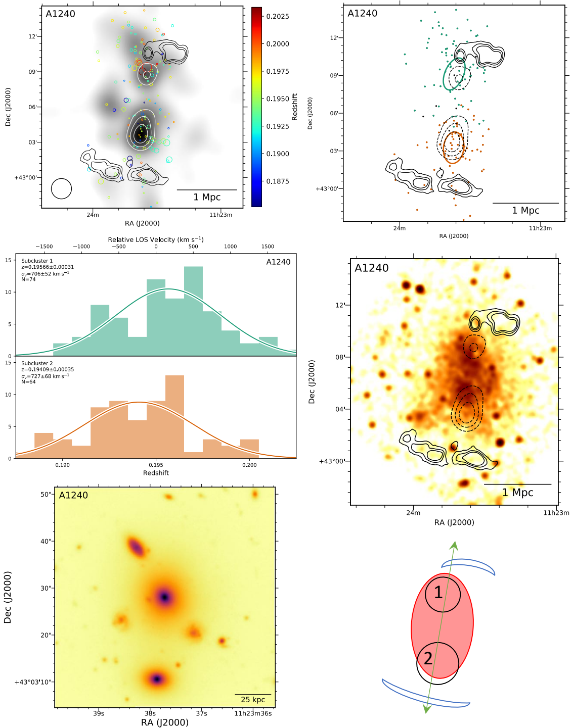
Figure 15. Abell 1240 Top left: DS-test over red sequence r-band luminosity distribution with linearly spaced white contours. The black contours show the 1.4 GHz VLA contours (Bonafede et al. 2009). Top right: Subcluster membership of spectroscopic cluster members assigned with our GMM analysis. The same VLA contours (solid) and red sequence luminosity contours (dashed) are depicted. Middle left: Subcluster redshift histograms with colors matching the image at the top right. Middle right: 52 ks Chandra image with the same VLA radio contours (solid) and red sequence luminosity contours (dashed). The relics and disturbed ICM are suggestive of a merger between subclusters 1 and 2. Bottom left: 150 kpc cutout of the Subaru/SuprimeCam r-band image centered on the southern BCG, which is associated with subcluster 2. Bottom right: Proposed merger scenario. A1240 is a clean bimodal merger with two radio relics colinear with the two subclusters.
