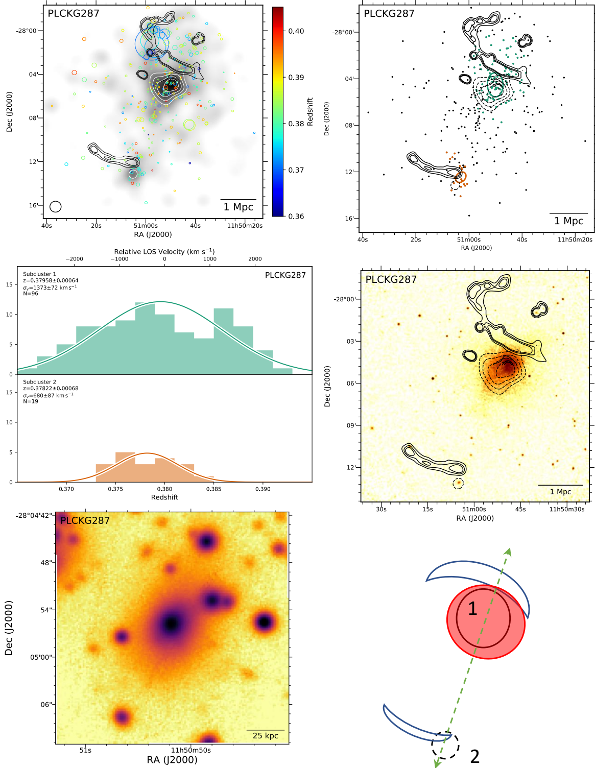
Figure 30. PLCK G287.0+32.9 Top left: DS-test over red sequence Subaru/SuprimeCam r-band luminosity distribution with linearly spaced white contours. The black contours show GMRT 325 GHz contours (Bonafede et al. 2014). Top right: Subcluster membership of spectroscopic cluster members assigned with our GMM analysis. The same GMRT contours (solid) and red sequence luminosity contours (dashed) are depicted. Middle left: Subcluster redshift histogram with colors matching the image at the top right. Middle right: 200 ks Chandra image with the same GMRT radio contours (solid) and red sequence luminosity contours (dashed). Bottom left: 150 kpc cutout of the Subaru i-band image centered on the cluster BCG in subcluster 1. Bottom right: Preferred merger scenario. The merger scenario is unclear. There is evidence for a small subcluster in the south near the southern radio relic; however, it leads the relic. There is disturbed X-ray emission streaming to the south of subcluster 1, which could motivate this merger scenario. A detailed weak gravitational lensing analysis detected composite structure in subcluster 1 (Finner et al. 2017), and more complex scenarios have been proposed (Bonafede et al. 2014).
