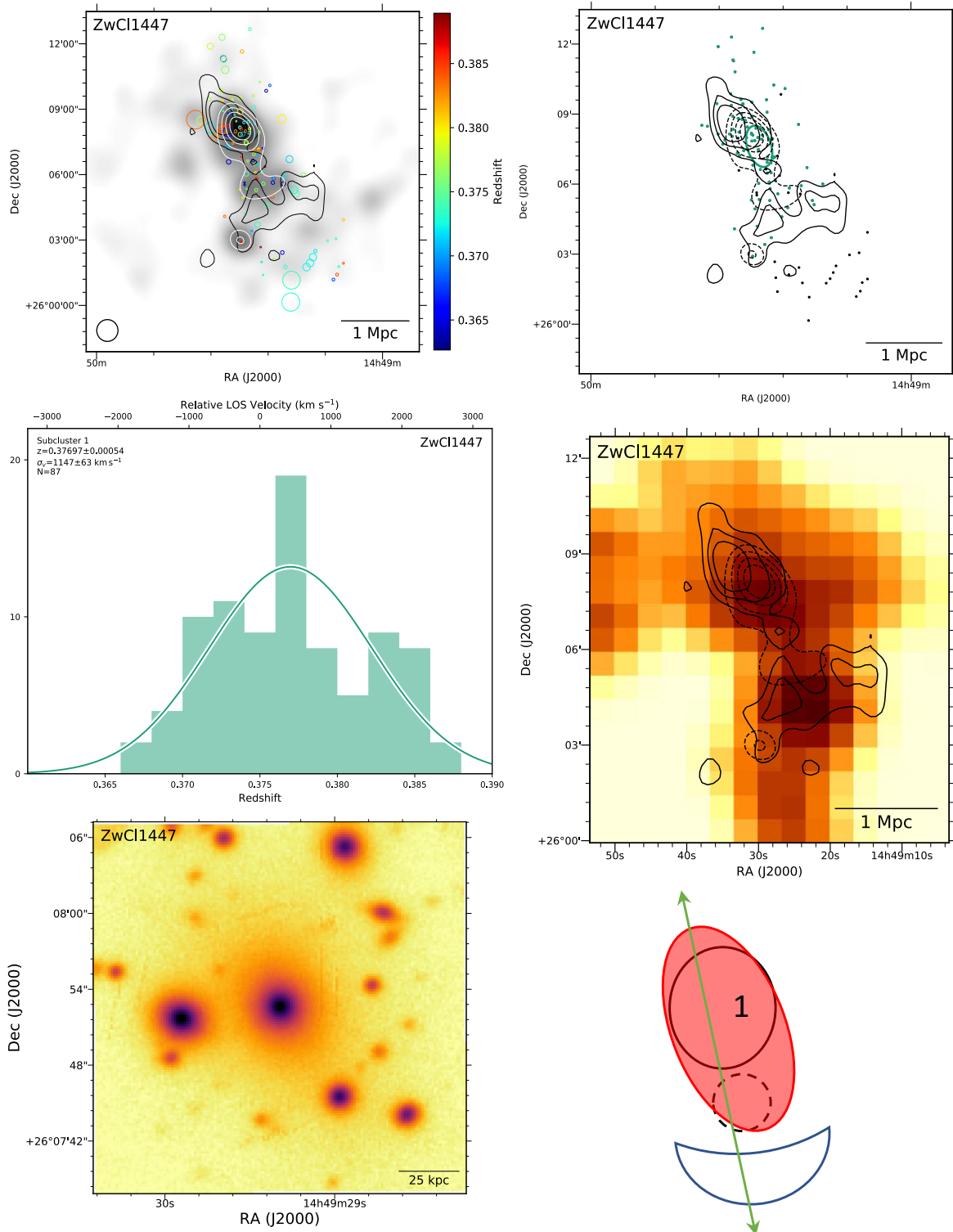
Figure 35. ZwCl 1447.2+2619 Top left: DS-test over red sequence Subaru/SuprimeCam r-band luminosity distribution with linearly spaced white contours. The black contours show VLA 1.4 GHz contours (Govoni et al. 2012). Top right: Subcluster membership of spectroscopic cluster members assigned with our GMM analysis. The same VLA contours (solid) and red sequence luminosity contours (dashed) are depicted. Middle left: Subcluster redshift histogram with colors matching the image at the top right. Middle right: 21 ks ROSAT image with the same VLA radio contours (solid) and red sequence luminosity contours (dashed). Bottom left: 150 kpc cutout of the Subaru r-band image centered on the cluster BCG. Bottom right: Preferred merger scenario. The GMM did not detect two subclusters; however, the red sequence luminosity is elongated along the same axis as the X-ray surface brightness and radio relics. We propose a north-south merger axis. Further spectroscopy in the south is necessary to better constrain the subcluster velocities.
