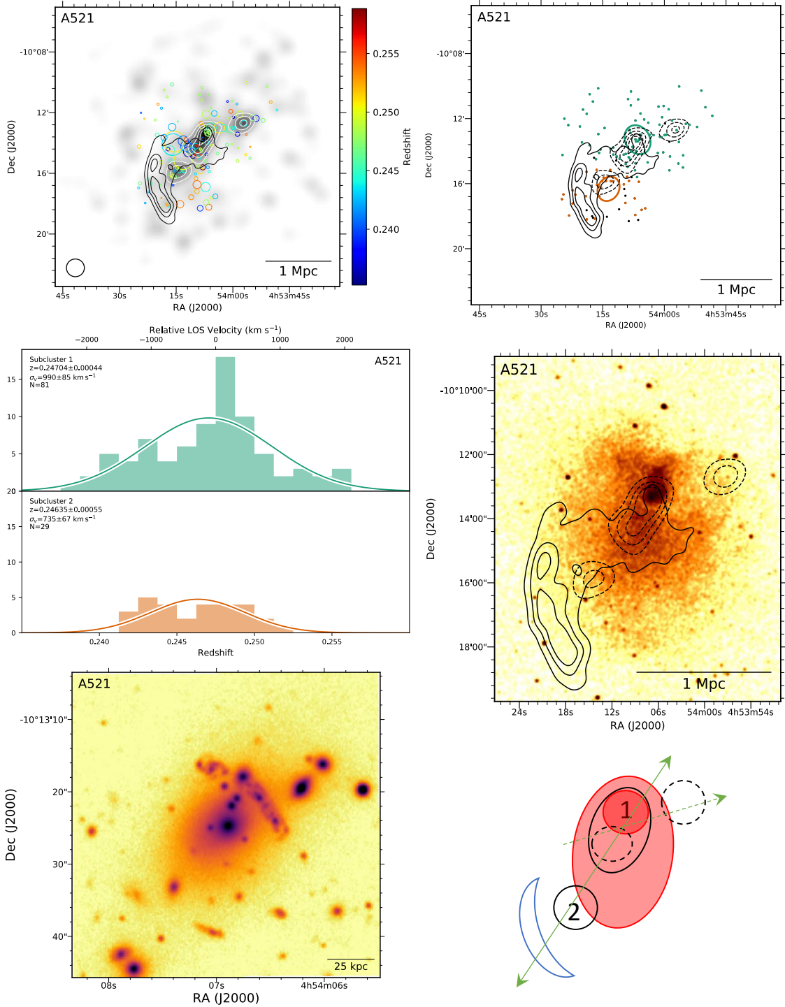
Figure 11. Abell 521 Top left: DS-test over red sequence i-band luminosity distribution with linearly space white contours. The black contours show the 240 MHz GMRT contours (Venturi et al. 2013). Top right: Subcluster membership of spectroscopic cluster members assigned with our GMM analysis. The same GMRT contours (solid) and red sequence luminosity contours (dashed) are depicted. Middle left: Subcluster redshift histograms with colors matching the image at the top right. Middle right: 170 ks Chandra image with the same GMRT radio contours (solid) and red sequence luminosity contours (dashed). A complex merger scenario is evident. Bottom left: 150 kpc cutout of the Subaru/SuprimeCam i-band image centered on the BCG of subcluster 1. The multiple images of the face on spiral are evident. Bottom right: Proposed merger scenario. Dashed black circles correspond to galaxy substructure not identified by the GMM analysis. The dark red region corresponds to the dense ICM core coincident with the BCG.
