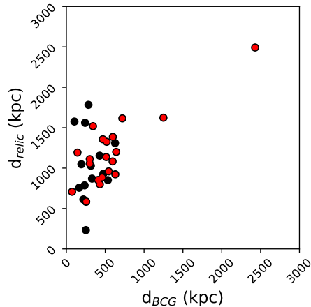
Figure 42. Projected distances from the center of mass to radio relics versus projected distance from the center of mass to the opposite subcluster BCG for 35 radio relics from 24 merging clusters (black) and 22 radio relics from 11 double radio relic systems (red). We find a correlation between these two parameters, as expected for a simple model of relic propagation in the center of mass frame. The correlation test is discussed in §6.3.
