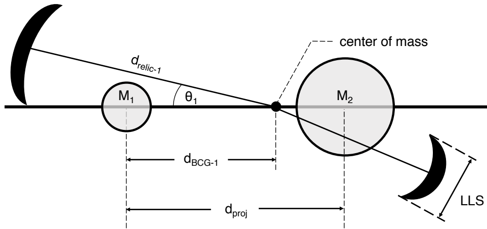
Figure 40. Schematic representation of the relic geometry for a double relic system (e.g. A1240). Each relic is located with a position angle and distance from the center of mass of the system determined from the velocity dispersions of subclusters aligned with the radio relics. Single relic systems follow the same conventions. LLS is an abbreviation for the largest linear scale of a radio relic, which is often quoted in radio astronomy literature and has been shown to correlate with the propagation distance of a shock.
