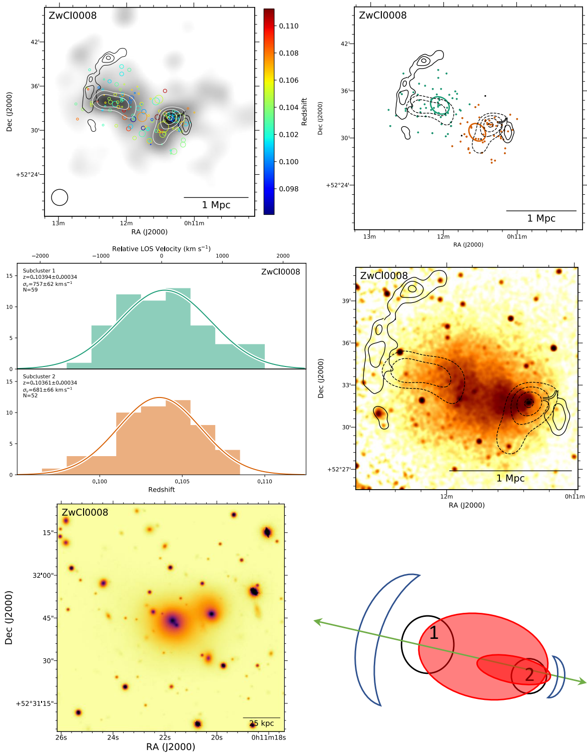
Figure 34. ZwCl 0008.8+5215 Top left: DS-test over red sequence Subaru/SuprimeCam r-band luminosity distribution with linearly space white contours. The black contours show WSRT 1382 MHz contours (van Weeren et al. 2011c). Top right: Subcluster membership of spectroscopic cluster members assigned with our GMM analysis. The same WSRT contours (solid) and red sequence luminosity contours (dashed) are depicted. Middle left: Subcluster redshift histogram with colors matching the image at the top right. Middle right: 411 ks Chandra image with the same WSRT radio contours (solid) and red sequence luminosity contours (dashed). Bottom left: 150 kpc cutout of the Subaru r-band image centered on the cluster BCG in subcluster 2. Bottom right: Preferred merger scenario. The two subclusters and radio relics are aligned with the extended X-ray emission. A ‘bullet’ like cool-core remnant and wake feature are associated with subcluster 2, which is traveling to the west. The cluster exhibits simple, bimodal geometry indicative of the Bullet Cluster.
