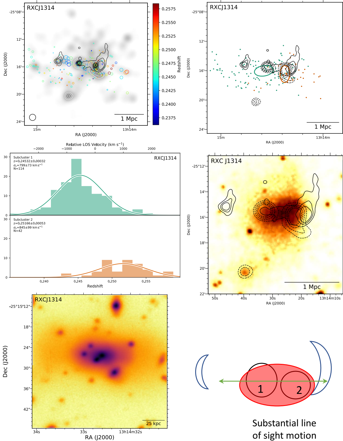
Figure 33. RXC J1314.4-2515 Top left: DS-test over red sequence Subaru/SuprimeCam r-band luminosity distribution with linearly spaced white contours. The black contours show VLA 2-4 GHz contours (P.I. Dawson). Top right: Subcluster membership of spectroscopic cluster members assigned with our GMM analysis. The same VLA contours (solid) and red sequence luminosity contours (dashed) are depicted. Middle left: Subcluster redshift histogram with colors matching the image at the top right. Middle right: 110 ks XMM image with the same VLA radio contours (solid) and red sequence luminosity contours (dashed). Bottom left: 150 kpc cutout of the Subaru r-band image centered on the cluster BCG in subcluster 1. Bottom right: Preferred merger scenario. The two subclusters and radio relics are aligned with the extended X-ray emission. A large line of sight velocity difference between the two subclusters is discovered suggesting a substantial component of the merger axis is along the line of sight, which is an outlier among other bimodal, double relic systems. A third subcluster is detected to the southeast, in the red sequence luminosity and X-ray surface brightness. It may have interacted in a glancing collision given the stream of X-ray emission connecting it to the cluster center.
