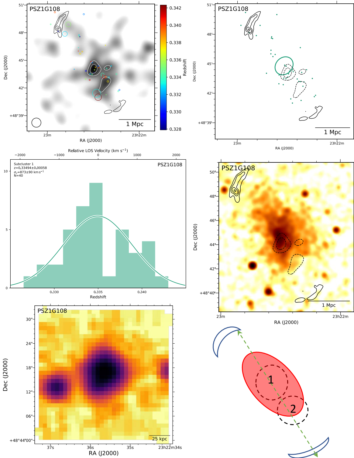
Figure 31. PSZ1 G108.18-11.53 Top left: DS-test over red sequence DSS R-band luminosity distribution with linearly space white contours. The black contours show GMRT 323 GHz contours (de Gasperin et al. 2015). Top right: Subcluster membership of spectroscopic cluster members assigned with our GMM analysis. The same GMRT contours (solid) and red sequence luminosity contours (dashed) are depicted. Middle left: Subcluster redshift histogram with colors matching the image at the top right. Middle right: 27 ks Chandra image with the same GMRT radio contours (solid) and red sequence luminosity contours (dashed). Bottom left: 150 kpc cutout of the DSS R-band image centered on the cluster BCG. Bottom right: Preferred merger scenario. We do not have enough spectra to resolve composite structure, but the red sequence luminosity is multi-modal and aligned with the two radio relics and extended X-ray emission. Since the X-ray, radio, and optical light is all aligned, we propose a simple bimodal merger along this axis.
