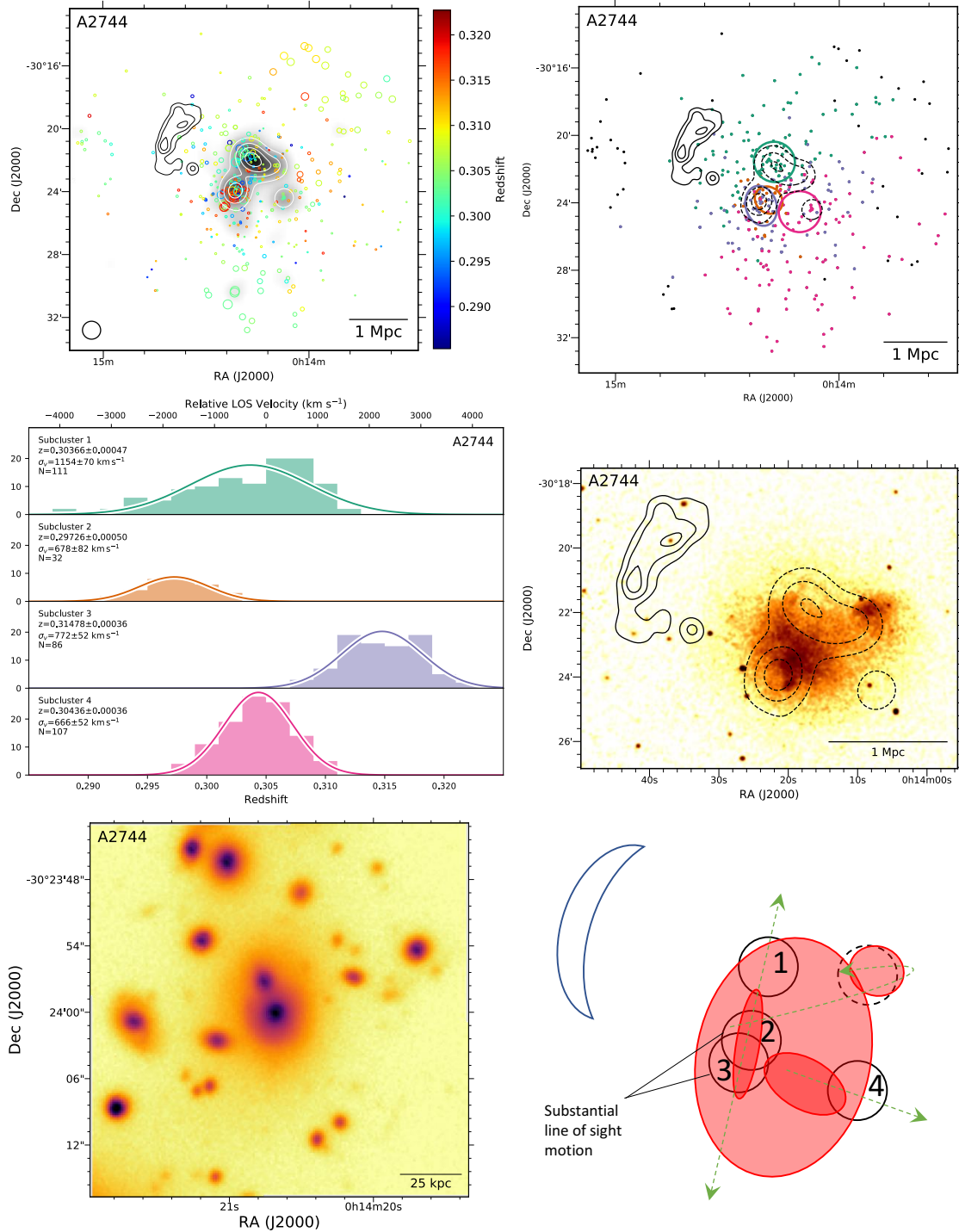
Figure 24. Abell 2744 Top left: DS-test over red sequence Subaru/SuprimeCam R-band luminosity distribution with linearly space white contours. The black contours show the 325 MHz GMRT contours (Venturi et al. 2013). Top right: Subcluster membership of spectroscopic cluster members assigned with our GMM analysis. The same GMRT contours (solid) and red sequence luminosity contours (dashed) are depicted. Middle left: Subcluster redshift histogram with colors matching the image at the top right. Middle right: 132 ks Chandra image with the same GMRT radio contours (solid) and red sequence luminosity contours (dashed). Bottom left: 150 kpc cutout of the Subaru/SuprimeCam R-band image centered on the cluster BCG in subcluster 2. Bottom right: Preferred merger scenario. A2744 is the most complex merger in our sample. The core of the cluster (subclusters 2 and 3) has been studied in detail as a HST Frontier Field and has a substantial line of sight motion. Subclusters 1 and 4 have been stripped of their ICM suggesting post merger scenarios. Finally, a fifth subcluster with an associated ICM further from the cluster than the galaxies suggests a ram-pressure slingshot type scenario.
