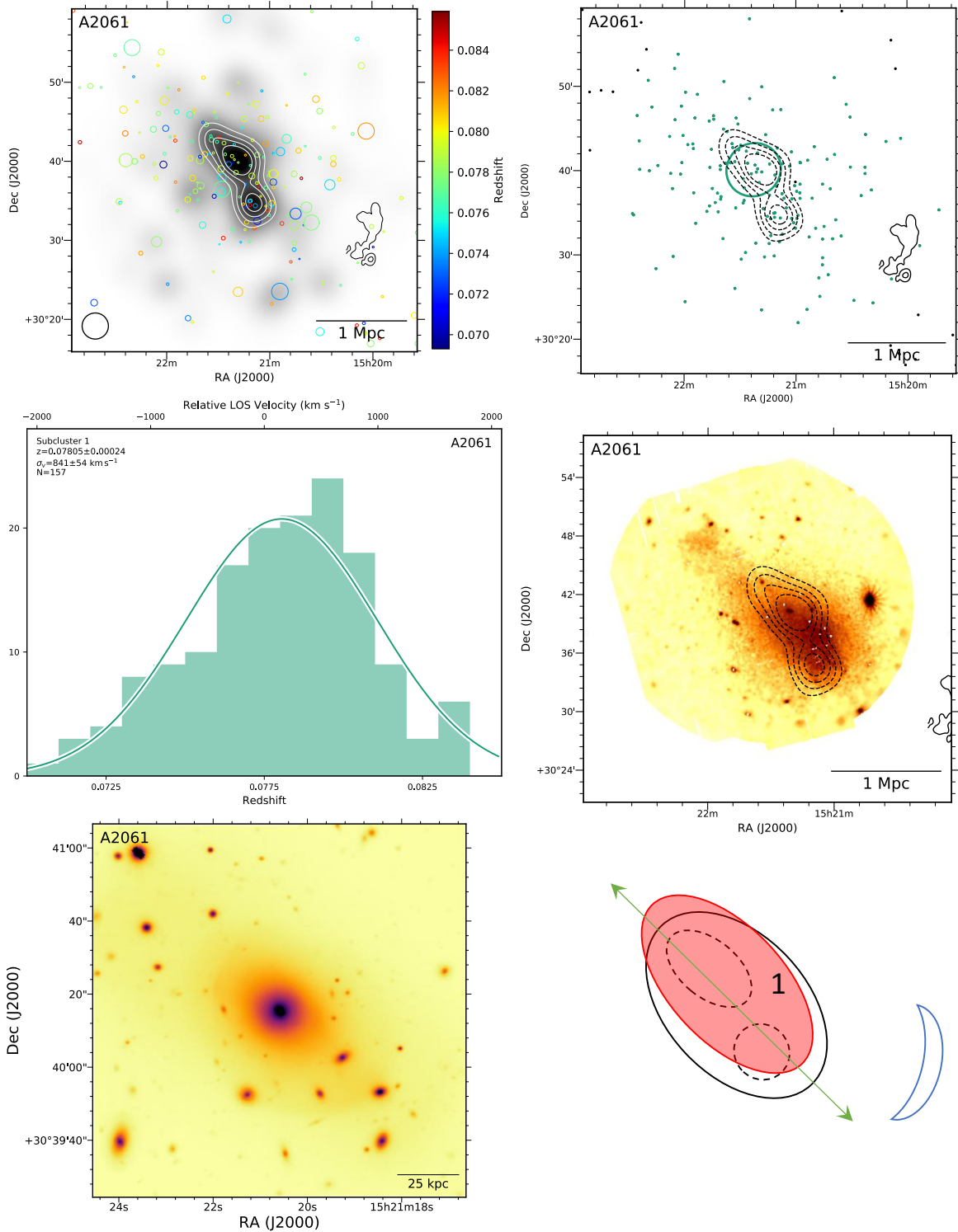
Figure 19. Abell 2061 Top left: DS-test over red sequence r-band luminosity distribution with linearly space white contours. The black contours show the 1.4 GHz WSRT contours (van Weeren et al. 2011b). Top right: Subcluster membership of spectroscopic cluster members assigned with our GMM analysis. The same WSRT contours (solid) and red sequence luminosity contours (dashed) are depicted. The small projected separation and low spectroscopic survey density likely contributes to a single halo model being preferred by the BIC analysis. Middle left: Subcluster redshift histograms with colors matching the image at the top right. Middle right: 50 ks XMM image with the same WSRT radio contours (solid) and red sequence luminosity contours (dashed). The relic at the edge of the frame in the southwest and the disturbed ICM are suggestive of a merger between at least two subclusters. The extended stream of X-ray emission to the northeast toward A2067 is unlikely due to a merger between the two. A2067 sits 2.7 Mpc away. Bottom left: 150 kpc cutout of the Subaru/SuprimeCam r-band image centered on the cluster BCG in the southwest. Bottom right: Proposed merger scenario. Two subclusters are apparent in multiple wavelengths, but the GMM is unable to separate them due to low spectroscopic sampling and a small projected separation.
