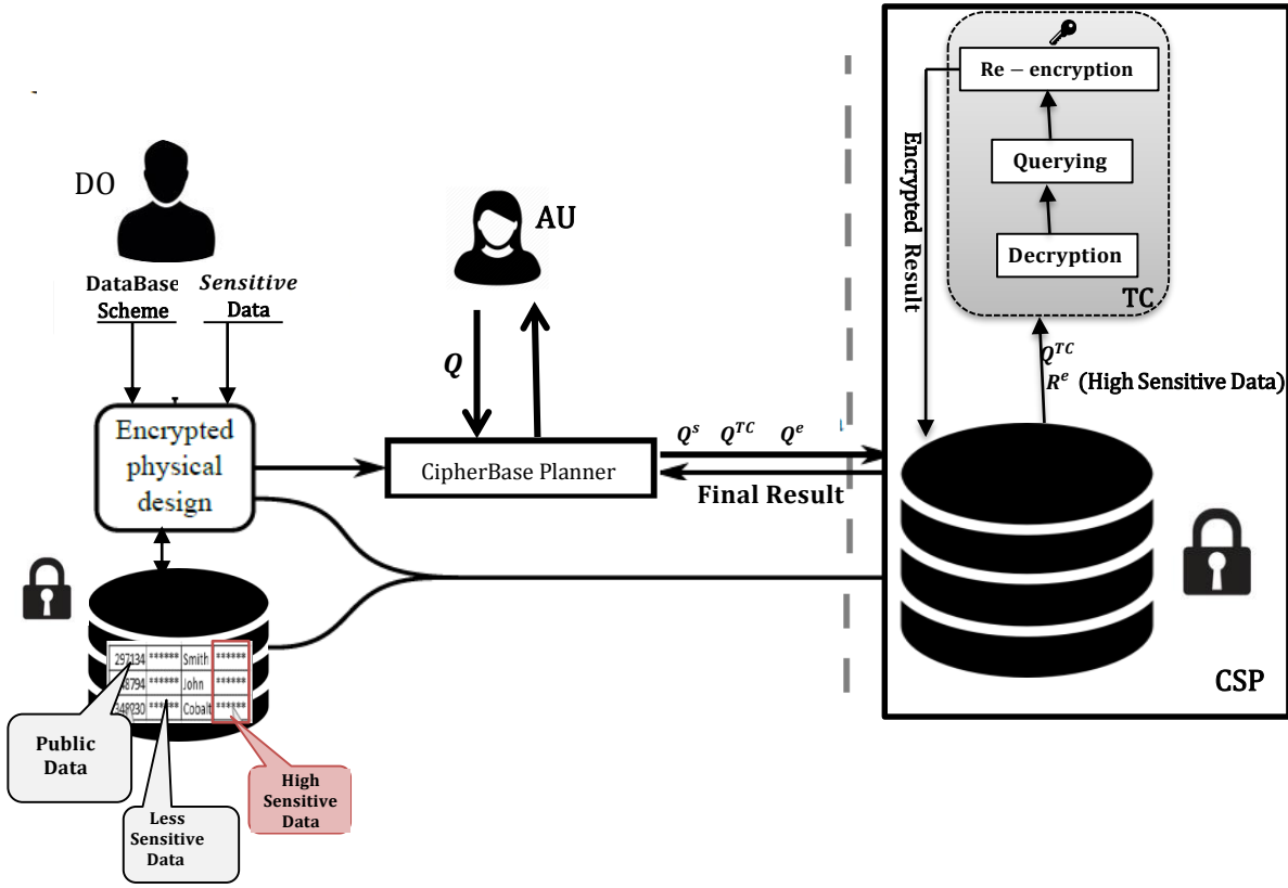
FIGURE 10. CipherBase architecture and query processing workload
