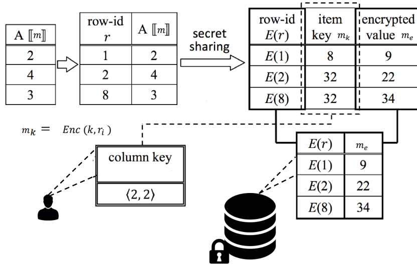
FIGURE 8. Encryption of attribute A in SDB [67]
