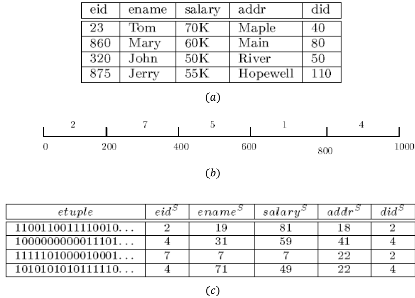
FIGURE 3. (a) An example of a relation R , (b) partition function used for attribute eid , and (c) the encryption relation R^S stored at the CSP [10]
