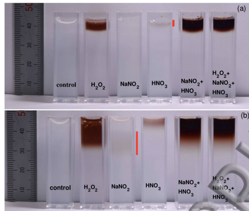
FIG. 5: Photographs of the KI-starch gel after 150 \mu l volumes of 1 mM H_2O_2 , NaNO_2 and HNO_3 or mixtures of these were dispensed on top of the gel and incubated for (a) 25 and (b) 60 minutes. The vertical red line on the right of the cuvette indicates the brown region in the cuvette for HNO_3 in (a) and in NaNO_2 (b). Control is KI-starch gel only.
