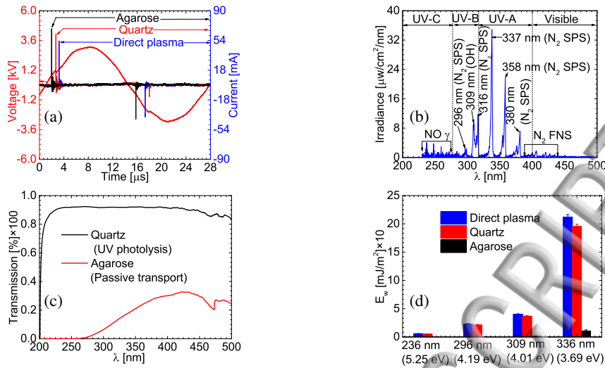
FIG. 2: (a) Electrical characteristics of the argon plasma jet (voltage and current waveforms) in contact with the DI water [Fig. 1(b)], quartz [Fig. 1(c)] and agarose [Fig. 1(d)]. (b) OES of the argon plasma jet operated into ambient air showing emissions for the visible, UV-A, UV-B and UV-C wavelength range. (c) Percentage transmittance for the quartz plate (UV photolysis) and agarose tissue model (passive transport). (d) Photon energy density delivered to the surface of the DI water ( E_w ) for water directly exposed to the plasma jet and indirectly through the quartz or agarose.
