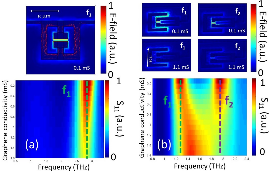
Figure 2. (a) COMSOL simulation of the SRR unit cell, with the E-field at resonance. Below is reported the S11 parameter at different values of graphene conductivity. (b) COMSOL simulation and E-field representation of the EIT unit calculated at frequency f_1 and f_2 for different values of graphene conductivity EM picture of the SRR arrays for the amplitude modulators. (b) SEM picture of a single resonant unit for the EIT device used for frequency modulation. The graphene patterned region, showed by the dashed area, short the gap in the dark resonators. (c) Schematic of the final device.
