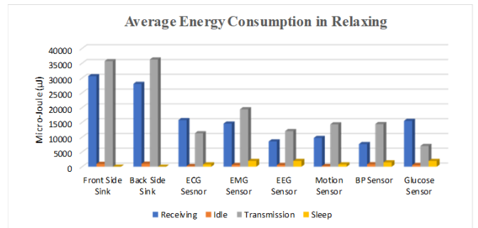
FIGURE 19. Average Energy Consumption during Relaxing.
