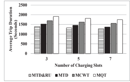
(c) Average Trip Duration
