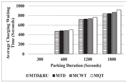
(a) Average Charging Waiting Time
