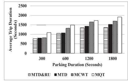
(c) Average Trip Duration
