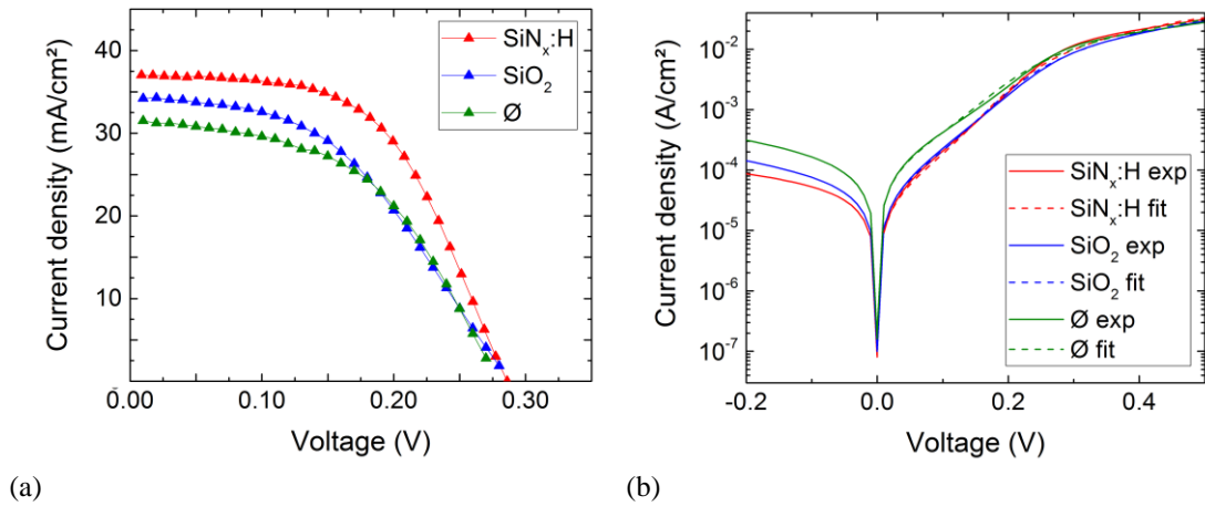
Fig.3 (a) Measured 1 sun JV curves for all types of control solar cells (5% shading factor): with SiN_x:H passivation (red), with SiO_2 passivation (blue) and without any passivation (green). (b) Measured (solid lines) and fitted (dashed lines) dark JV curves for all types of control solar cells (5% shading factor): with SiN_x:H passivation (red), with SiO_2 passivation (blue) and without any passivation (green).
