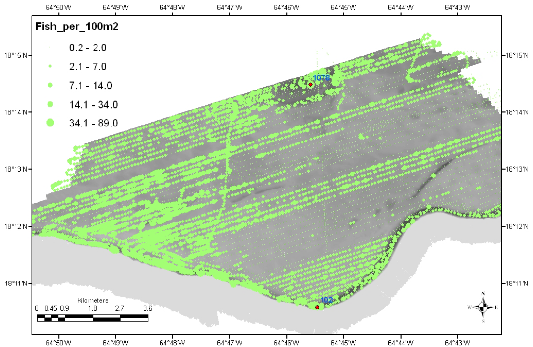
Figure 23. Fish density (fish/100m 2 ) at Virgin Passage (upper) and St. John shelf (lower).
