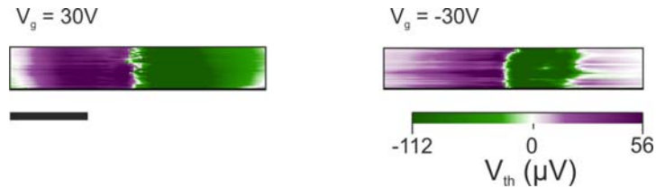
Figure S12. Gate dependent thermovoltage measurements. Global thermovoltage recorded as the hot tip is scanned over a bow tie device at two different back gate voltages V_g = 30V and V_g = -30V .
