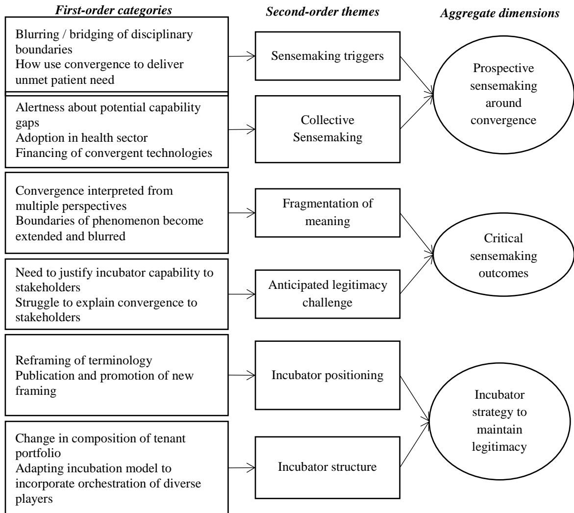
Figure 1. Data structure
