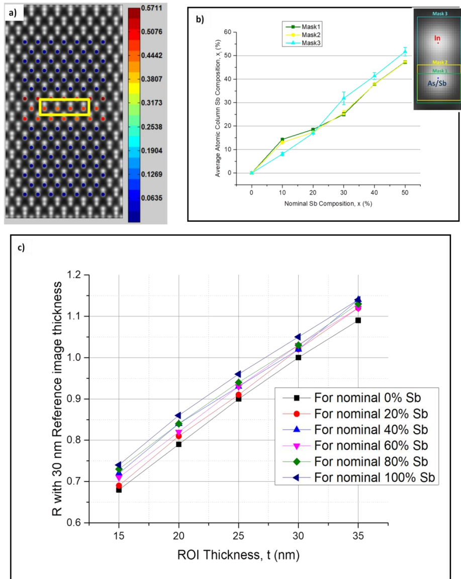
Figure 3 (a) Atomic column composition map calculated from the modified qHAADF originated 'R' values shown in Figure 2b, superimposed to the HAADF-STEM simulated image. (b) Graph of the average atomic column Sb composition calculated from the modified qHAADF originated 'R' values vs. the nominal Sb composition for the three masks considered. The error bars illustrates standard deviations to the corresponding averages. The inset represents the three mask areas considered: Mask1 (green), Mask2 (yellow) and Mask3 (cyan), surrounding a single In-As/Sb dumbbell. (c) Plots of Sb composition induced R vs specimen thickness effect as per simulated HAADF-STEM signals with ROI thicknesses of 15-35 nm in association to average reference thickness of 30 nm.
