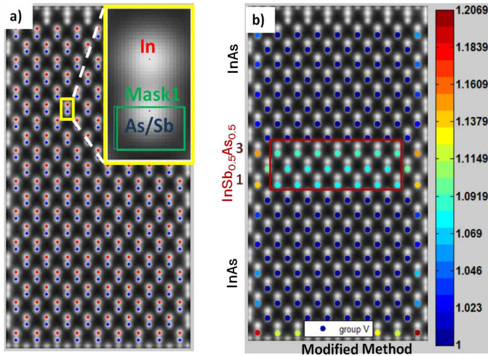
Figure 2 (a) HAADF-STEM simulated image of \text{InSb}_{0.5}\text{As}_{0.5} where the group III (In) atomic columns are marked with red dots and the group V (As/Sb) atomic columns with blue dots. The inset represents a single dumbbell where a group V atomic column is surrounded by a Mask1 (green rectangle). (b) The modified qHAADF method generated 'R' map corresponds the image in a). The red rectangle represents the \text{InSb}_{0.5}\text{As}_{0.5} area.
