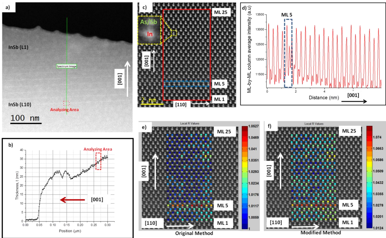
Figure 4 (a) Low-mag HAADF-STEM image where the red rectangle depicts the location of the analyzing ROI and Reference areas; (b) corresponding thickness profile associated to the Spectrum image line (green line), along with the analyzing area in Fig. 4a. (c) Experimental HAADF-STEM image of InSb/InAs (single In-As/Sb dumbbell at the inset); (d) intensity profile obtained from the image in Fig. 4c, evidencing the position of the InSb layer; R map calculated with the original (e) and modified (f) methods, from the HAADF-STEM image in Fig. 4c.
