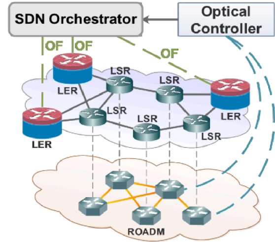
Fig. 10. A high-level view of a hierarchical SDN control architecture, including the main components
