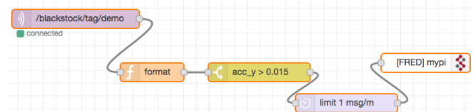
Figure 3. Flow to receive data from sensor tag, and send alert to a Raspberry Pi
