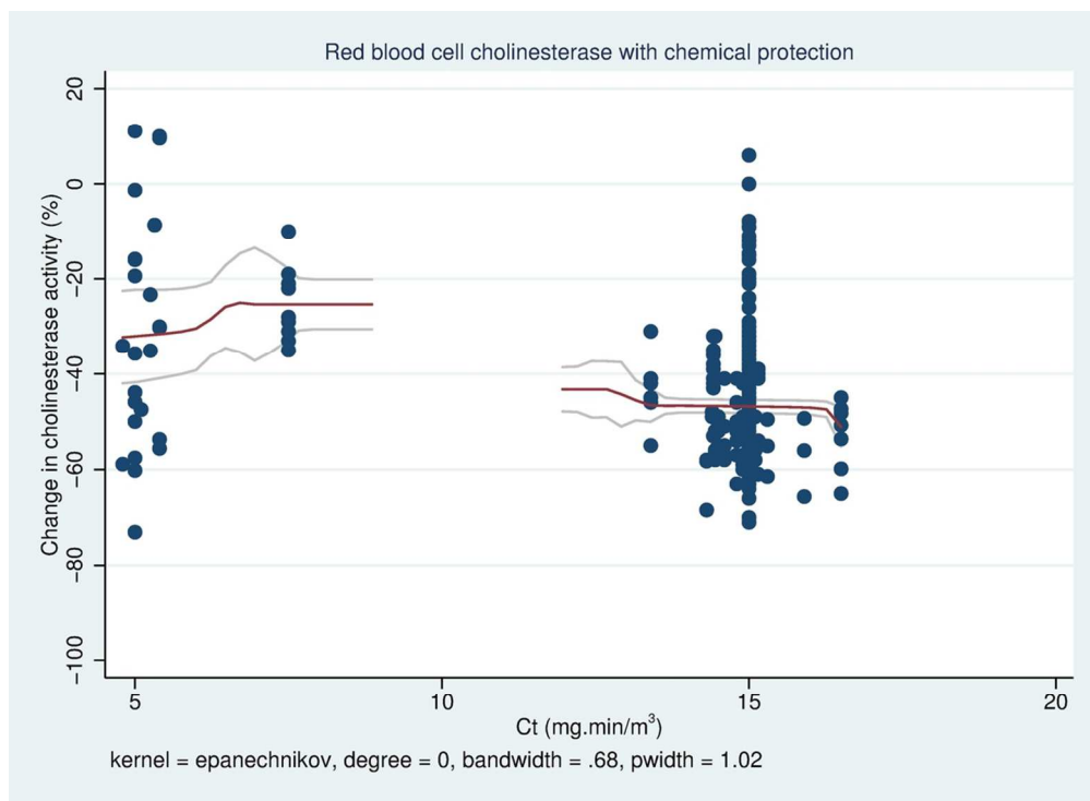
31 32 33 34 Figure 2 Non-parametric kernel regression estimate and 95% CIs for sarin inhalation exposure and percentage change in red blood cell cholinesterase activity, with a) chemical protection (n = 326) and b) no protection (n = 332).
