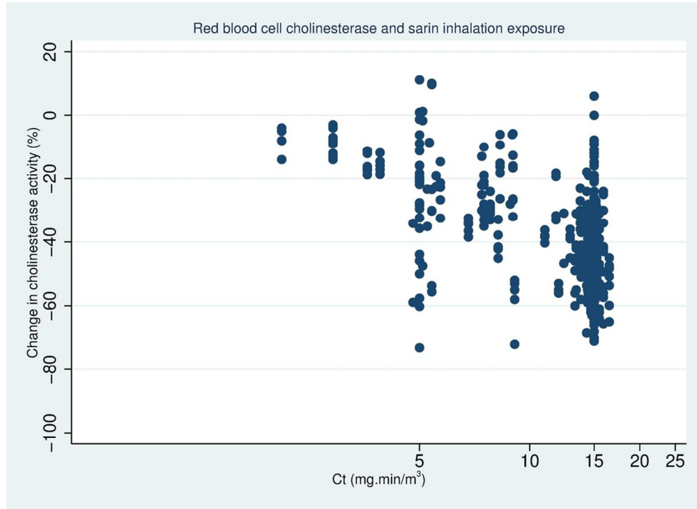
Figure 1 Scatter plots of sarin inhalation exposure and percentage change in activity of a) red blood cell, b) plasma, c) whole blood, and d) unspecified cholinesterase. e) Sarin dermal exposure and percentage change in activity of unspecified cholinesterase.
