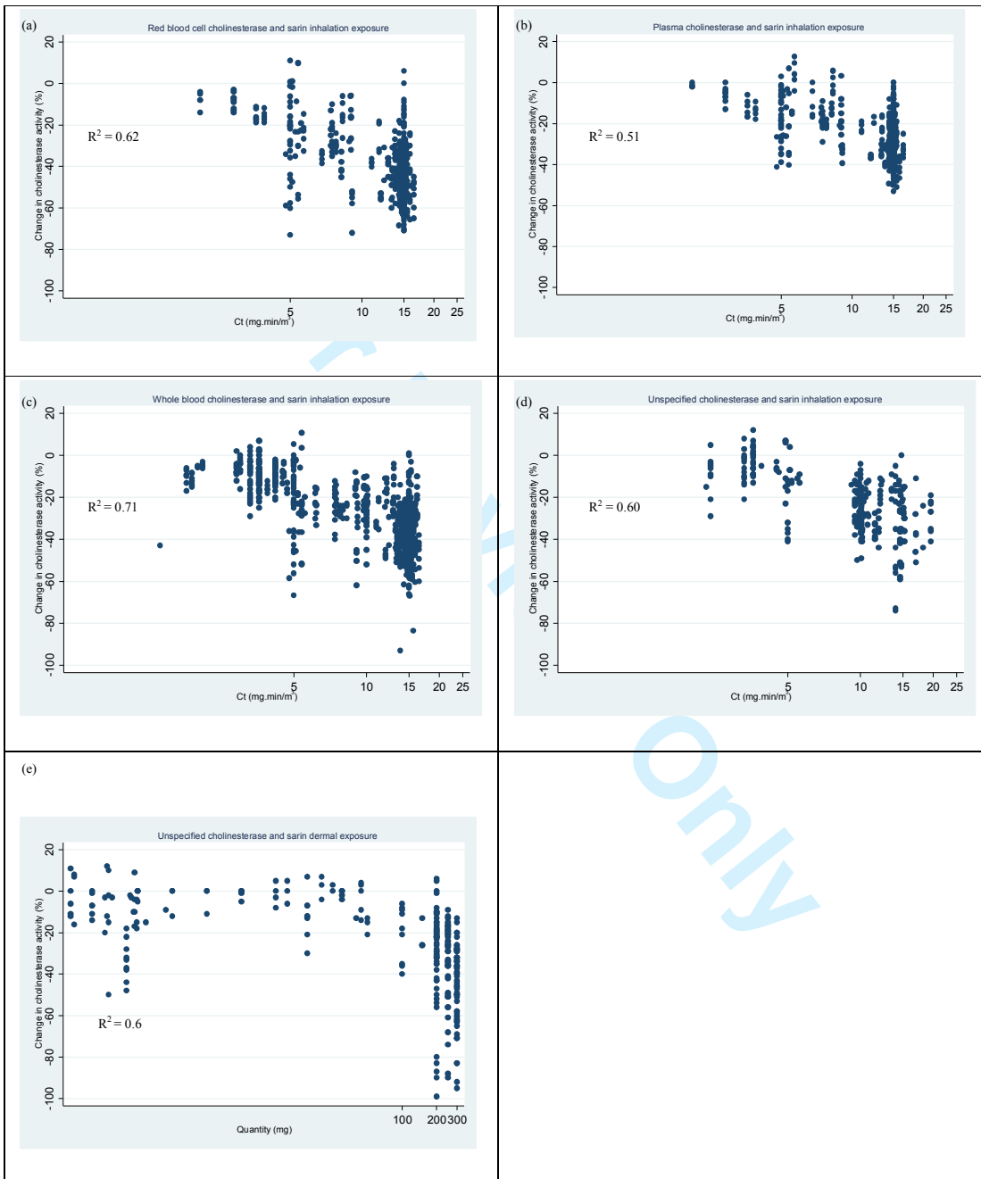
Figure 1 Scatter plots of sarin inhalation exposure and percentage change in activity of a) red blood cell, b) plasma, c) whole blood, and d) unspecified cholinesterase. e) Sarin dermal exposure and percentage change in activity of unspecified cholinesterase.
