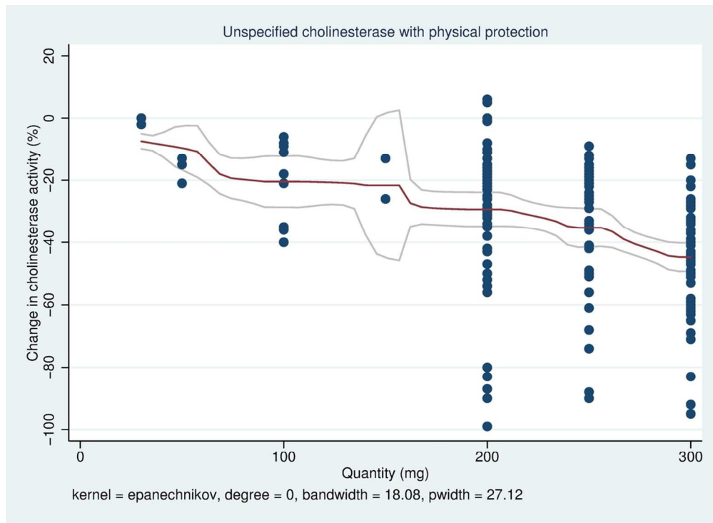
Figure 3 Non-parametric kernel regression estimate and 95% CIs for sarin dermal exposure and percentage change in unspecified cholinesterase activity, with a) physical protection (n = 185), and b) no protection (n = 88).
