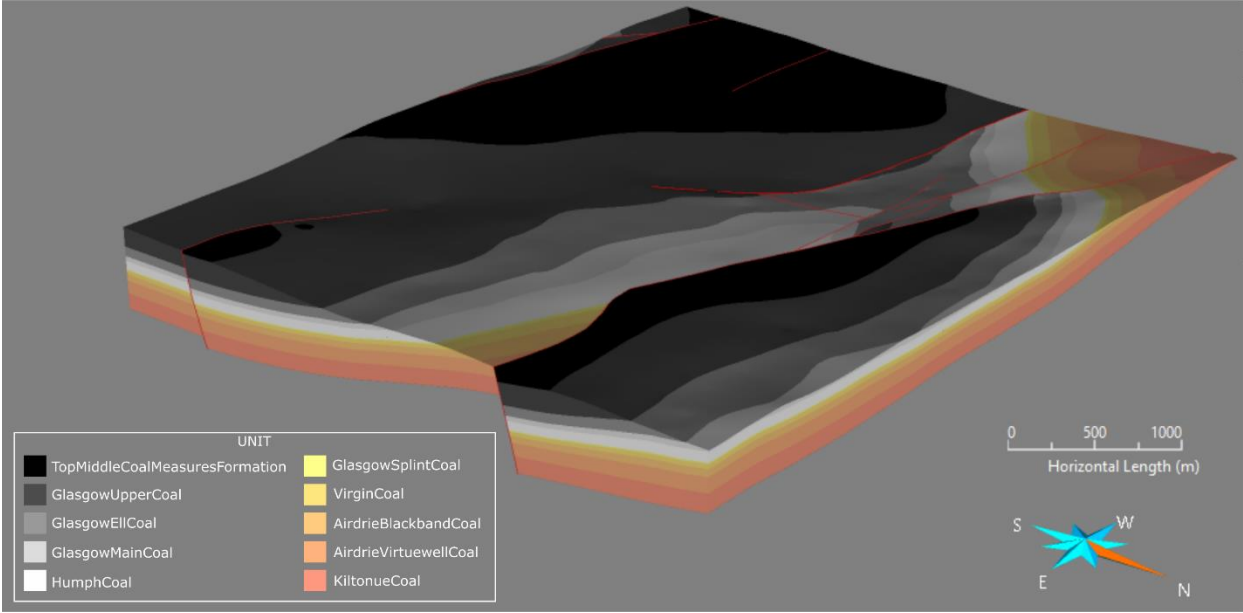
Figure 4 SKUA geological bedrock model, looking SW, vertical exaggeration X2. Top view on rockhead surface with superficial deposits removed.
