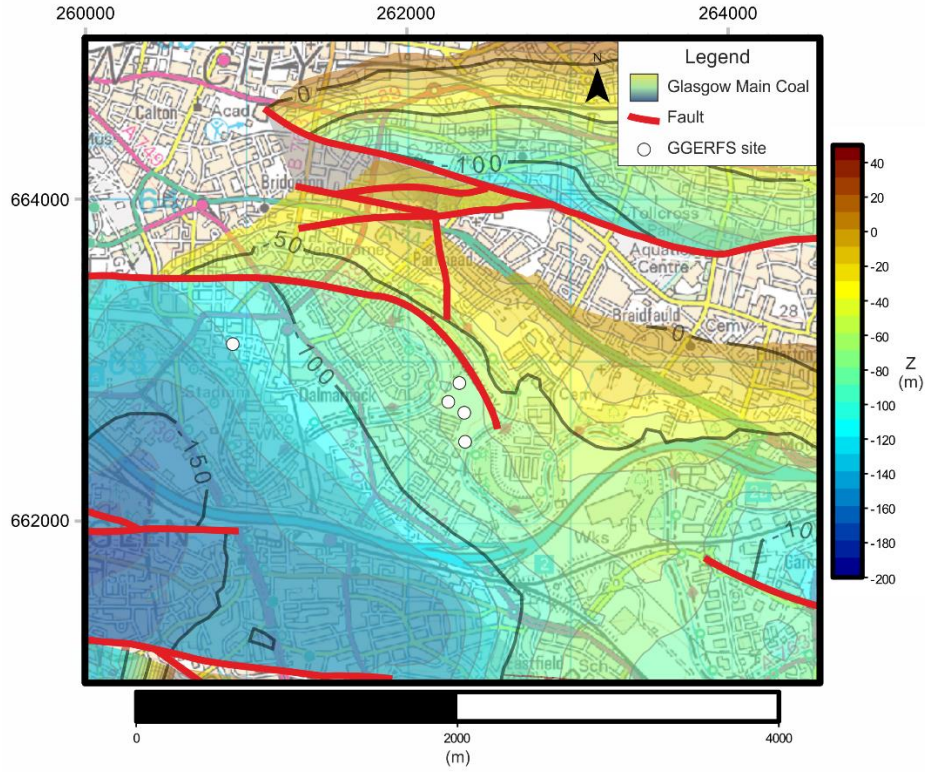
Figure 5 Contoured depth grid (m relative to Ordnance Datum) for the base of Glasgow Main Coal, horizon exported from the geological model showing the closed synclinal structure and variety of fault trends. Created using ArcGIS. Copyright © Esri. All rights reserved. Contains Ordnance Survey data © Crown copyright and database rights. All rights reserved [2019] Ordnance Survey [100021290 EUL].
