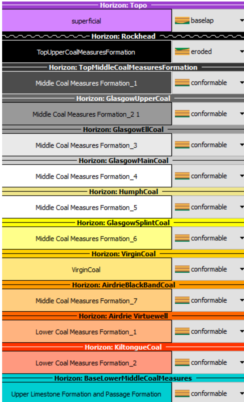
Figure 1 Stratigraphic column showing the modelled surfaces.
