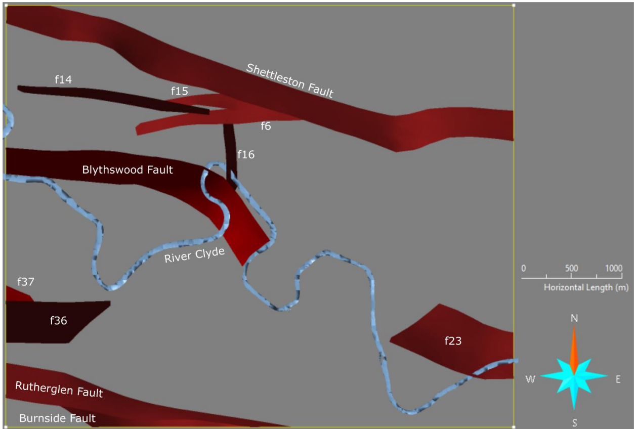
Figure 2 Modelled faults within the GGERFS study area. Note the truncation of many of the faults by the model extent boundary. River Clyde is shown for geographic reference.
