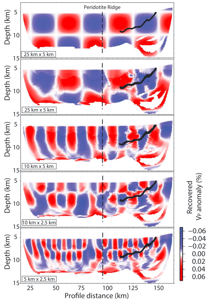
Figure 9. Checkerboard resolution test results. (top) Input velocity anomalies for the 25 \times 5 km checkerboard in order to demonstrate the boundaries between cells. Recovered velocity anomalies from the checkerboard tests are below. (second from top to bottom) The anomaly dimensions are 25 \times 5 km, 10 \times 5 km, 10 \times 2.5 km, and 5 \times 2.5 km, horizontally and vertically, respectively. Vertical dashed line indicates the axis of the Peridotite Ridge. Plots have a vertical exaggeration of 4.5.
