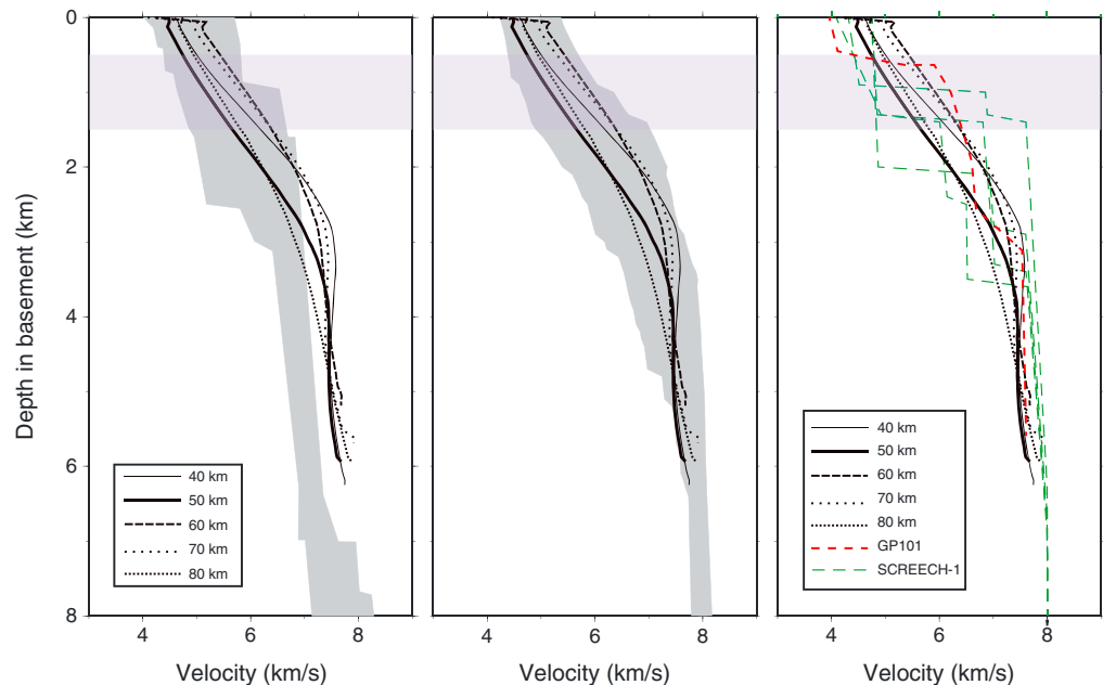
Figure 12. The 1-D velocity profiles through the final TOMO2D velocity model (Figure 5). Light blue shading indicates the depths at which the Moho, below oceanic crust, is identified. (left) The 1-D velocity profiles compared to the velocity envelope for Atlantic oceanic crust aged 59–170 Ma [White et al. , 1992]. (middle) The 1-D velocity profiles compared to the velocity envelope for velocity models within the COT from previous studies, as compiled by Minshull [2009]. (right) The 1-D velocity profiles compared with velocity profiles through thin oceanic crust on the SCREECH-1 compressional velocity model of Funck et al. [2003] (green dashed lines) and the GP101 model of Whitmarsh et al. [1996] (red dashed line).
