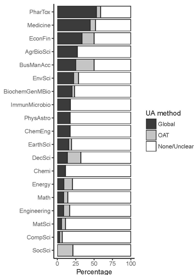
Fig. 5. Classification of uncertainty analysis by subject identifier, sorted by proportion of global methods.
