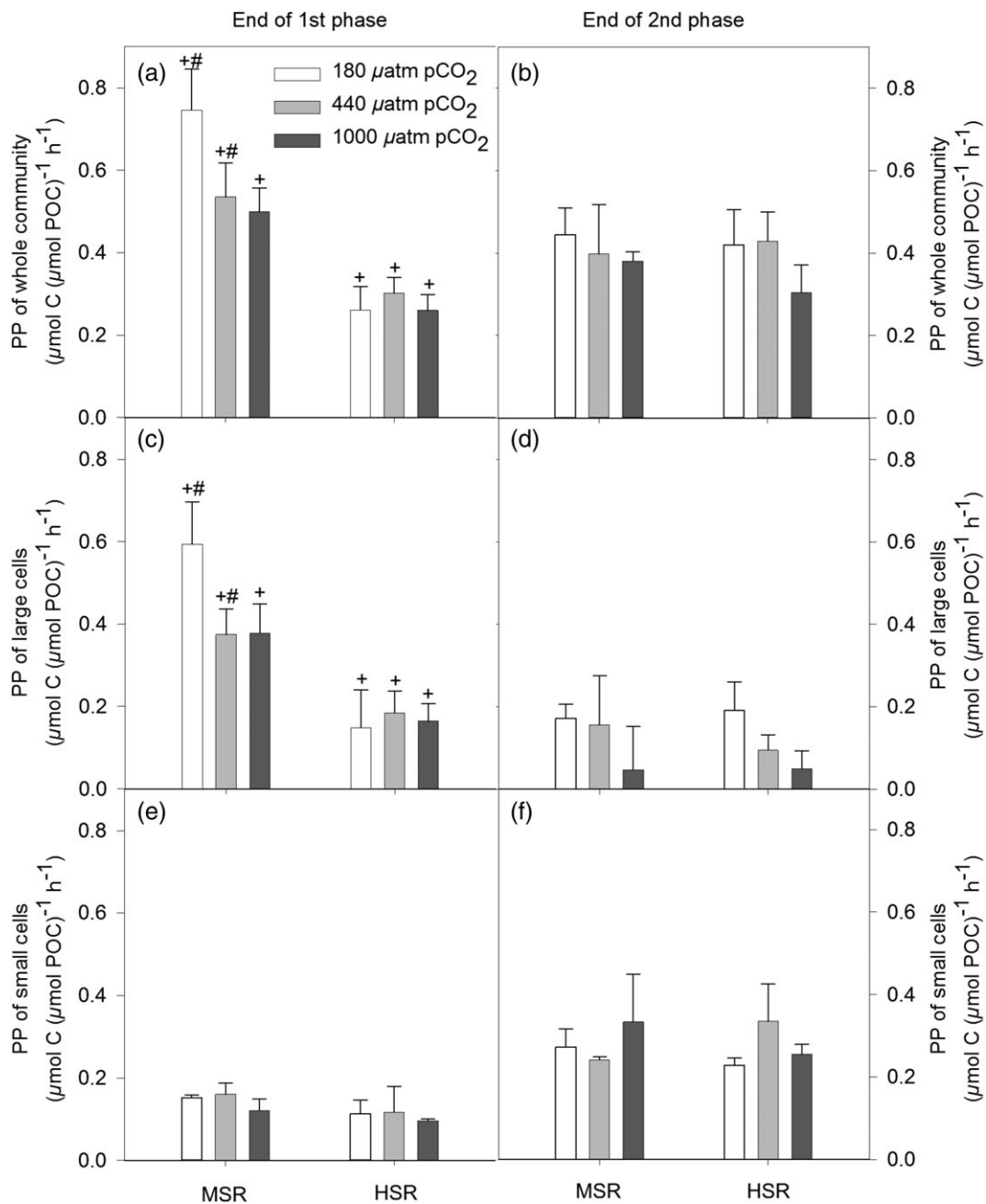
Fig. 2. Net PP rates ( \mu\text{mol C } [\mu\text{mol POC}]^{-1} \text{ h}^{-1} ) of the whole community (a, b), of large ( >20 \mu\text{m} ; c, d) and small ( <20 \mu\text{m} ; e, f) cells from a natural phytoplankton community after the first (a, c, e) and the second (b, d, f) experimental phase after exposure to MSR and HSR in combination with low, ambient, and high pCO 2 . Values represent the means ( \pm SD) of triplicate incubations. Significant differences ( p < 0.05 ) between treatments are indicated by + for light effects and # for pCO 2 effects.
