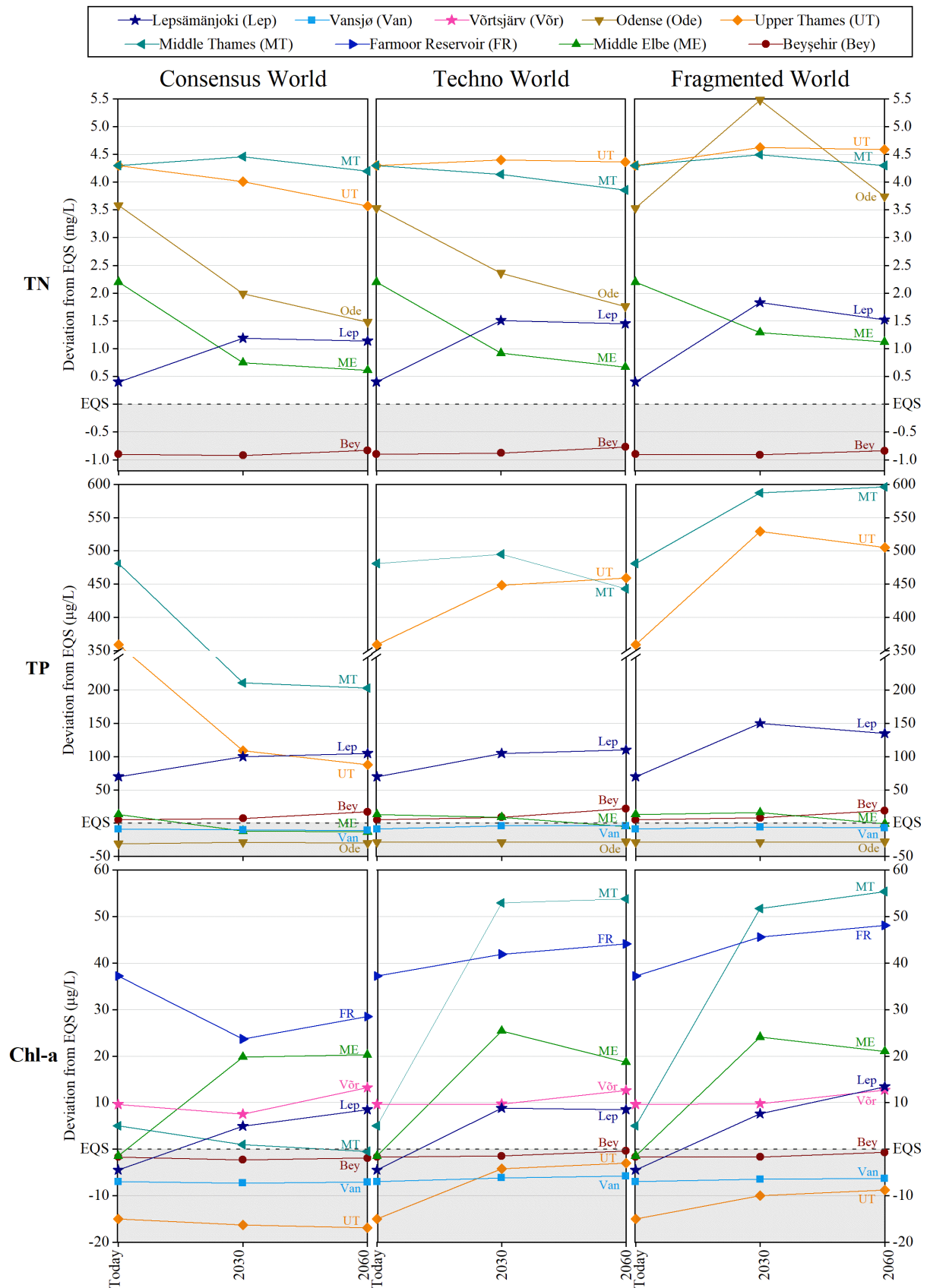
Figure 2: Modeled baseline and future concentrations of total nitrogen (TN), total phosphorus (TP) and chlorophyll-a (Chl-a), relative to the ecosystem type-specific threshold concentrations for good ecological status (EQS). The differences between the storylines are shown, highlighting a higher risk of failing the EQS for the Techno and Fragmented than for the Consensus World. Grey fields mark concentrations supporting the achievement of good ecological status.
