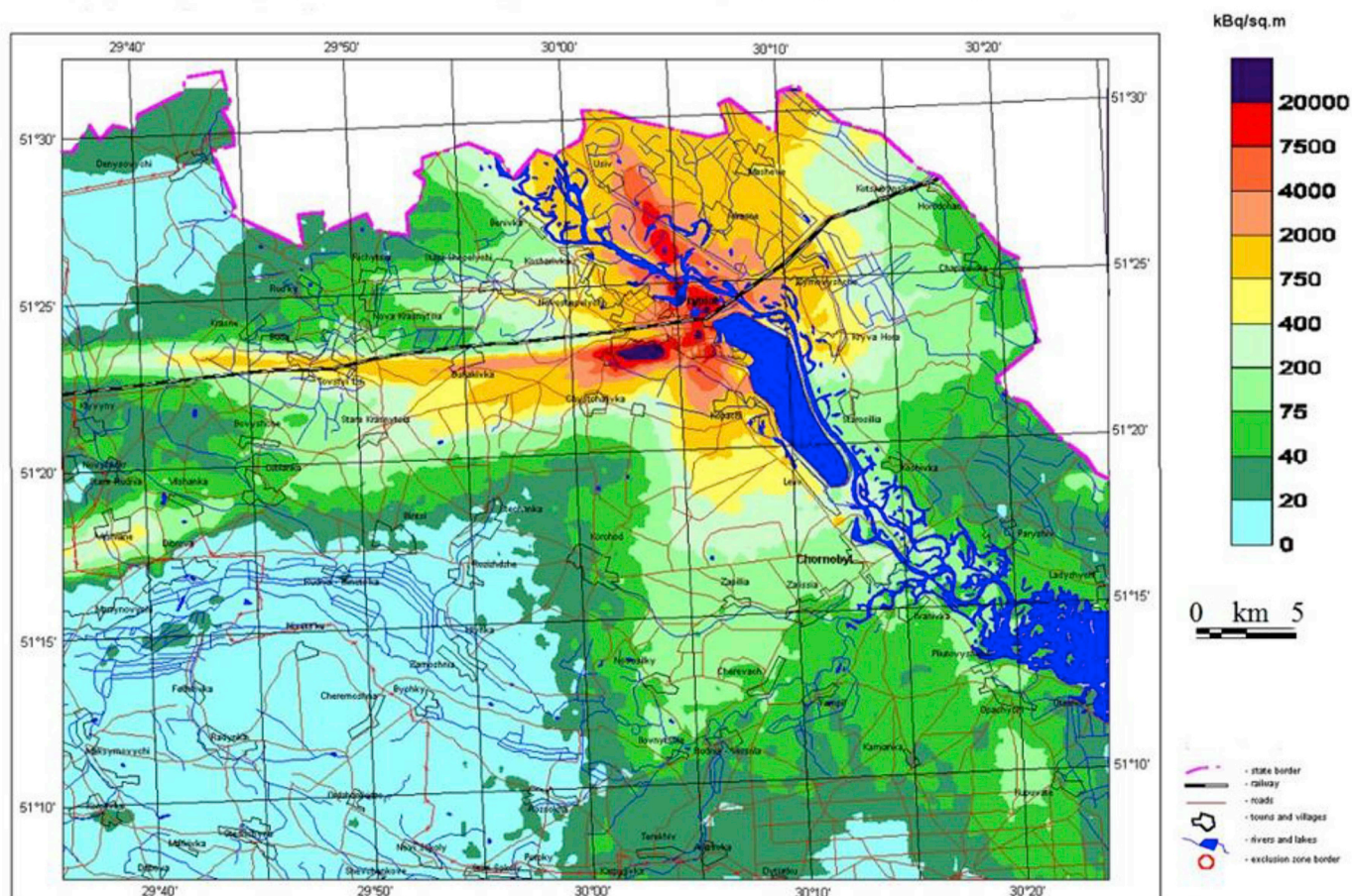
Fig. 1. Spatial pattern of ^{90}\text{Sr} contamination ( \text{kBq m}^{-2} ) estimated for 1997 (UIAR, 1998).
