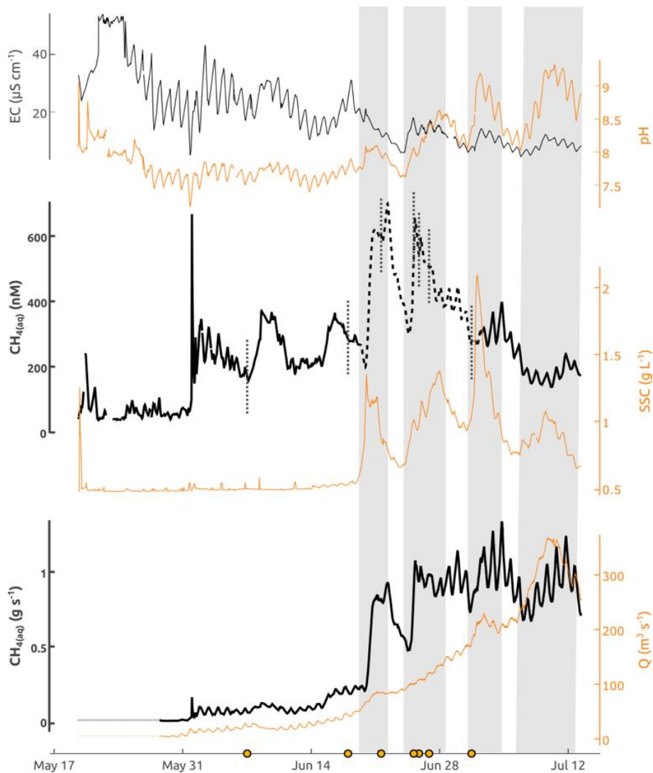
Fig. 1 Geochemical time series of the LG proglacial river – Top : Electrical-conductivity (EC) and pH. Middle : \text{CH}_{4(\text{aq})} (HydroC ® ) and suspended sediment concentrations (SSC); the dashed section corresponds to times when the HydroC ® sensor experienced slower response times (see Supplementary Information 2a, Extended Data Fig. 2). Orange dots and vertical dashed lines indicate sampling time of waters used for stable isotope analysis (see Extended Data Table 2). Bottom : \text{CH}_{4(\text{aq})} lateral flux and discharge (Q); the first data points on May 28 are extended to the first data point of the above sensor measurements (dashed horizontal lines). Abrupt increases in SSC, EC, pH, and \text{CH}_{4(\text{aq})} correspond to outburst events (shaded sections) and reflect sudden drainage of sub-ice sheet waters and sediments driven by supraglacial melt water entering the subglacial system (Supplementary Information 2b). Y axes corresponding to black and orange datasets are located on the left and right, respectively.
