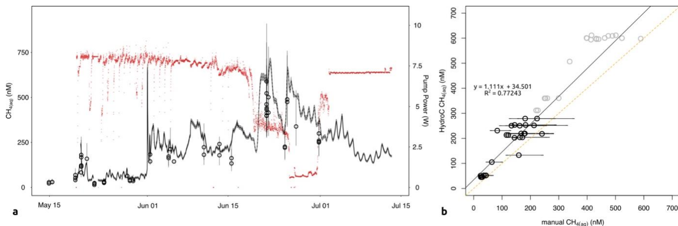
Extended data Fig. 2 | Comparison of CONTROS HydroC ® and manual sample \text{CH}_{4(\text{aq})} concentrations. a \text{CH}_{4(\text{aq})} time-series; red points correspond to the CONTROS HydroC ® pump power during operation. Continuous line depicts CONTROS HydroC ® measurements with the dashed section corresponding to times when the sensor experienced low pump power and thus a reduced water flow induced by the pump (~ June 19 to July 01); open circles correspond to manual samples. The thin shaded grey area ribbon around the \text{CH}_{4(\text{aq})} time-series corresponds to the uncertainty of the CONTROS HydroC ® measurements ( \sim \pm 3\% ); uncertainty on manual measurements indicated through error bars reflects error on vial internal pressures and volumes ( 119 \pm 0.76 mL standard deviation; internal pressures are derived from volumes, see Methods for details). b Regression plot between the CONTROS HydroC ® and manual sample measurements. Only manual samples taken during times where CONTROS HydroC ® pump power was above \sim 7\text{W} were considered for the regression (black circles, black line); grey circles correspond to samples taken during times of lower pump power. Horizontal error bars reflect errors on manual measurements; vertical error bars are smaller than size of circles. Orange line depicts a hypothetical 1:1 relationship between the sensor and manual measurements.
