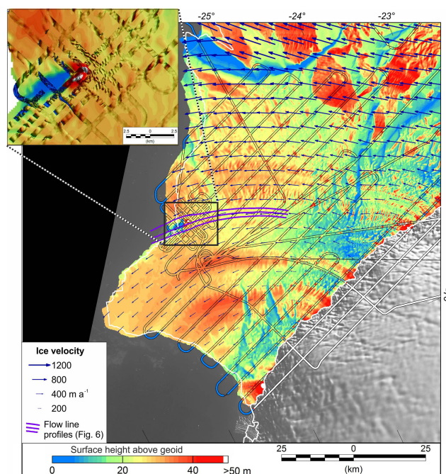
Figure 5. High-resolution surface digital elevation model (DEM) from WorldView surface height above the geoid (subsamped at 250 m × 250 m) for December 2016. This is cross-calibrated with airborne lidar data from the 2017 airborne campaign referenced to WGS84, then corrected to the same reference grid as the DEM by applying the BEDMAP2 geoid correction to obtain surface elevations above sea level. The effective timestamp of the surface DEM is 15 January 2017. Survey flight lines are marked by thin black lines. The velocity field is represented by blue arrows, based on data from June 2015. Purple lines mark the position of the flow lines plotted in Fig. 6. The white line marks the grounding line/ice shelf edge from the 2013 Antarctic Digital Database. The background image is a Landsat 8 image from 28 January 2017. The inset shows details of surface topography over the MIR region. Colour shaded data mark the full lidar swath gridded at 10 m. Note the complex pattern of ridges upstream and fractures downstream from the peak elevations, which mark the MIR pinning point.
