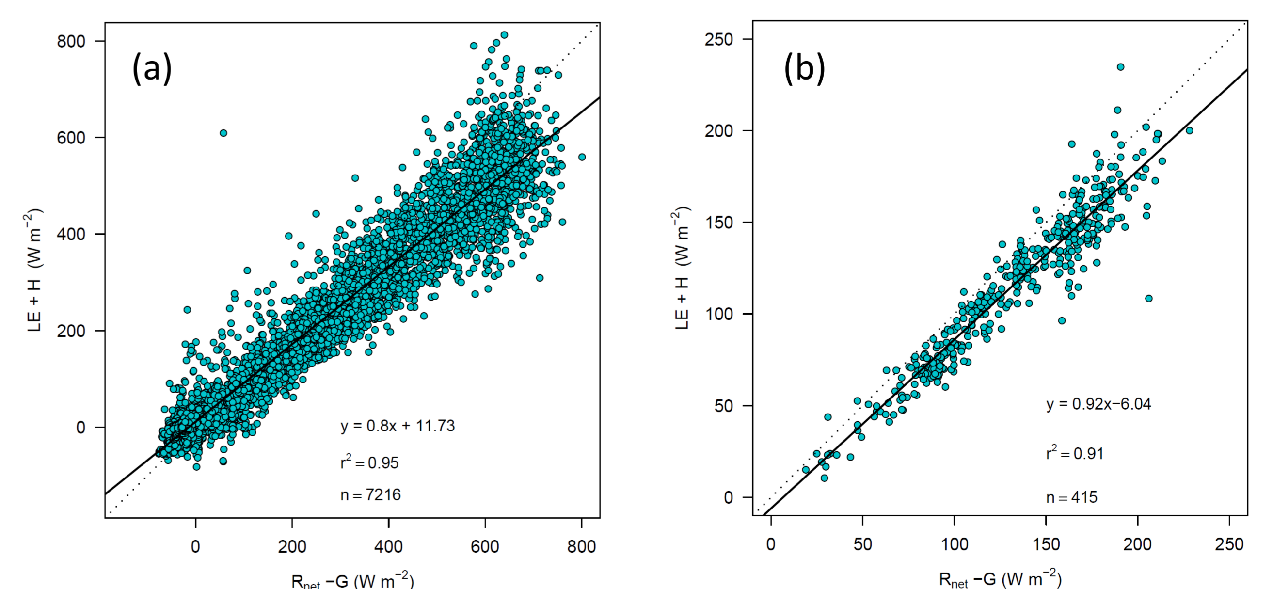
Figure 4. Surface energy balance closure evaluated using (a) thirty minute and (b) daily mean flux observations.
