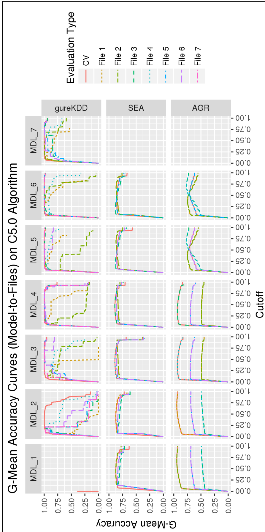
Figure A1. The gAcc curves for the C5.0 algorithm (see Table A1).
