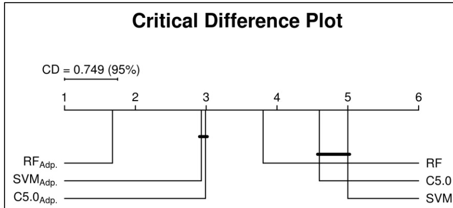
Figure 7. Critical differences plot of the pairwise Nemenyi comparison test for the cut-off (threshold) adaptation experiment.
