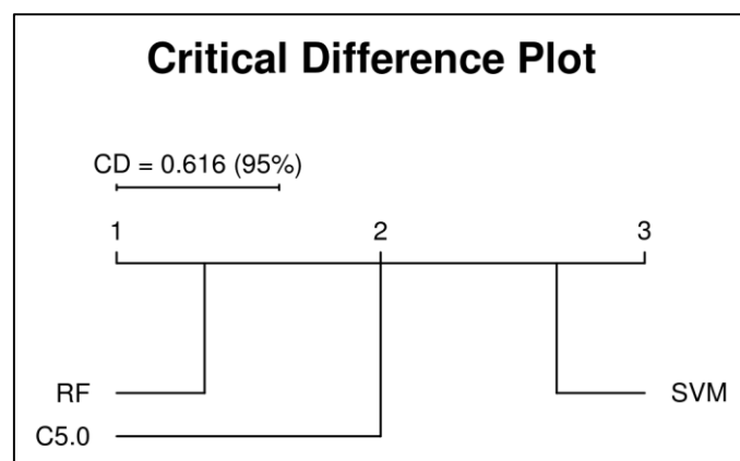
Figure 6. Critical differences plot of the pairwise Nemenyi comparison test for the full datasets 10-folds cross-validation experiment.
