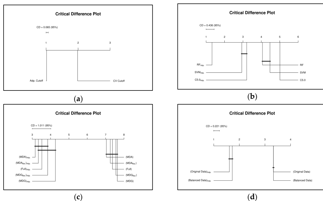
Figure 9. Graphical illustration of pairwise comparisons from the Friedman Test results for different threshold effects (optimal or adaptive cut-off) after applying the Nemenyi test (95% confidence level)
