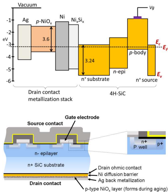
Fig. 13. Band energy alignment diagram and associated simplified SiC DMOSFET device structure, indicating the position of the NiO x layer that appeared on the back of the drain contact metallization stack.
