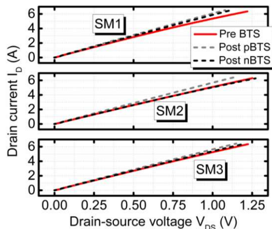
Fig. 8. Representative measured output characteristics for the three different SiC MOSFET types before and after the +20 V pBTS and -5 V nBTS constant gate bias stress tests at 300 °C for 30 minutes. Measurements were taken at room temperature and V_{gs} = +20 V.
