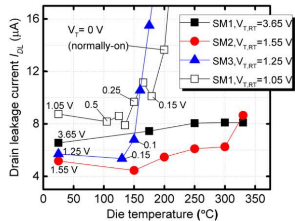
Fig. 9. Measured drain-source leakage currents versus die temperature for three different SiC MOSFET types, measured at V_{ds} = 10 V, V_{gs} = 0 V. The associated room temperature threshold voltage values ( V_{T,RT} ) are also shown. The leakage levels are heavily dependent on V_{T,RT} and increase exponentially when V_T \leq 150 mV approximately.
