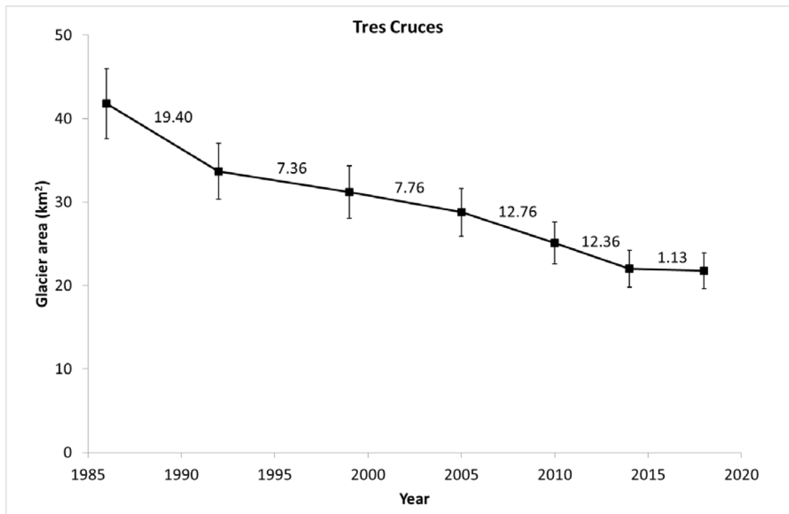
Fig. 3.6. Glacier area (km 2 ) and areal change (superimposed numbers on the graph in %) across the Bolivian Cordillera Oriental. Error bars are determined using Eq. (1) and represent an uncertainty of \pm 10\% .
