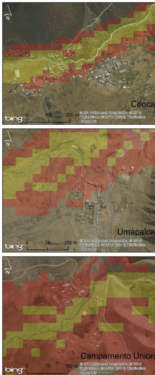
Fig. 3.15. GLOF impacts (from potential future lakes) on three communities in the Cordillera Real. Yellow=optimistic scenario. Red = pessimistic scenario.
