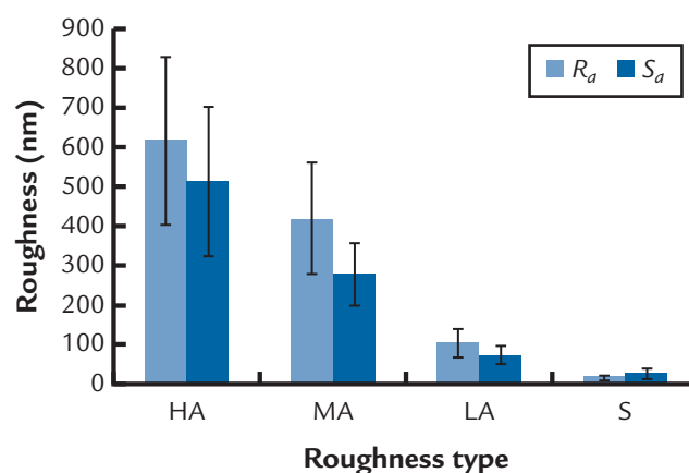
1 Surface roughness values ( S_a and R_a ) for abraded substrata with white light profilometry ( S_a values) and atomic force microscopy ( R_a values). S_a , average deviation of the roughness irregularities from the surface mean center line; R_a , average deviation of the roughness irregularities from the surface; HA, high abrasion; MA, medium abrasion; LA, low abrasion; S, smooth nonabraded (control).
