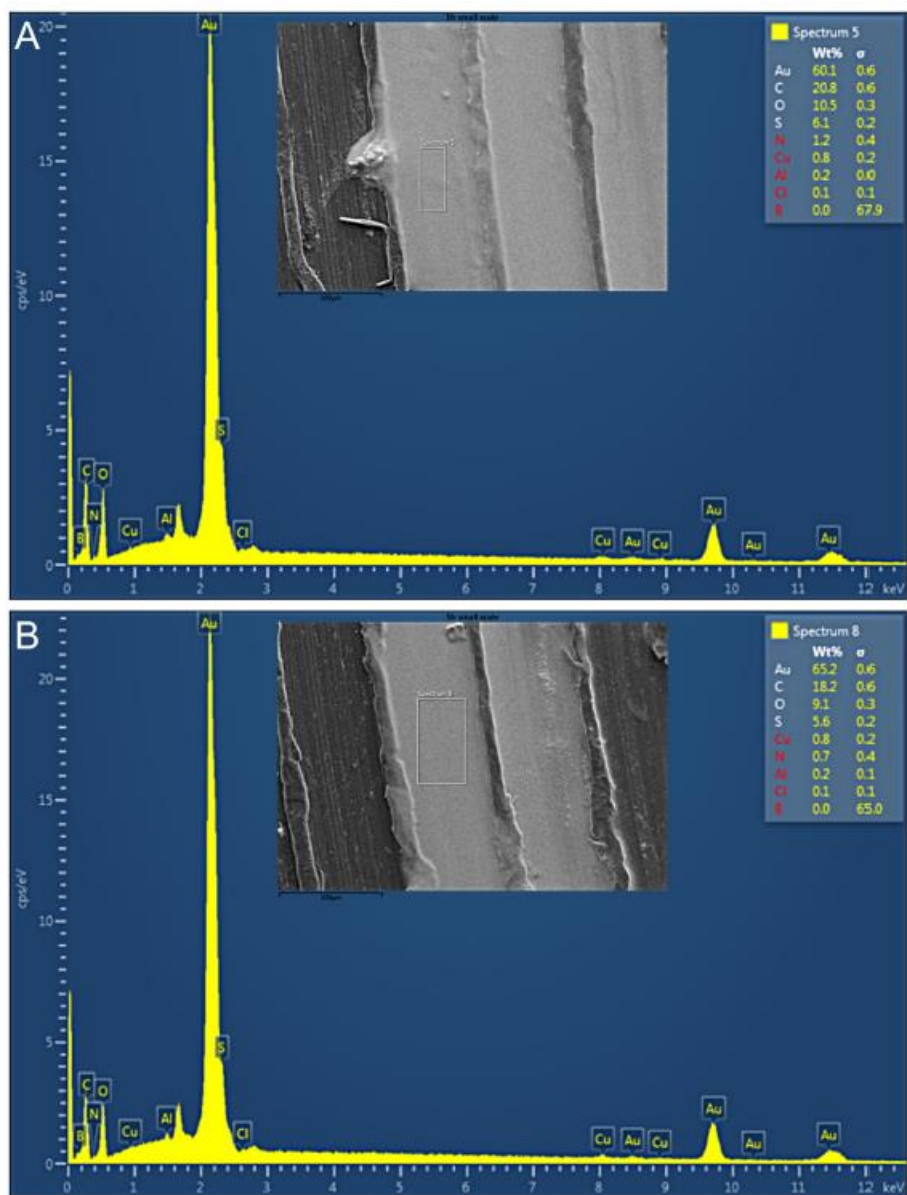
Figure 4.11: Elemental analysis of A. 1h synthesis time AuNP and B. 5h synthesis time AuNP as calculated by S: Au ratio on SEM. Representative spectra from a single run are shown with element peaks marked. Inserts represent SEM images showing the region analysed for each spectrum.
