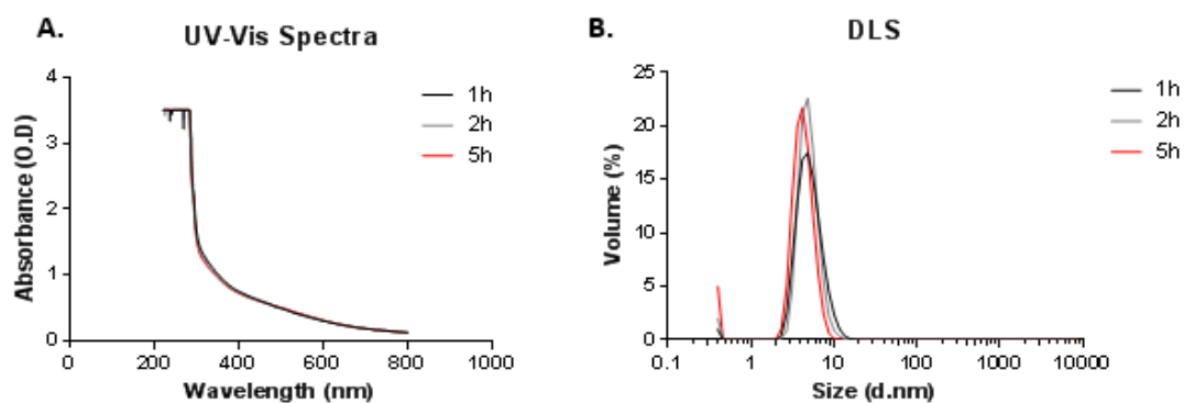
Figure 4.5: AuNPs physicochemical characterization for 1h, 2h and 5h synthesis time. A. UV-Vis spectra and B. Average hydrodynamic diameter measured by DLS.
