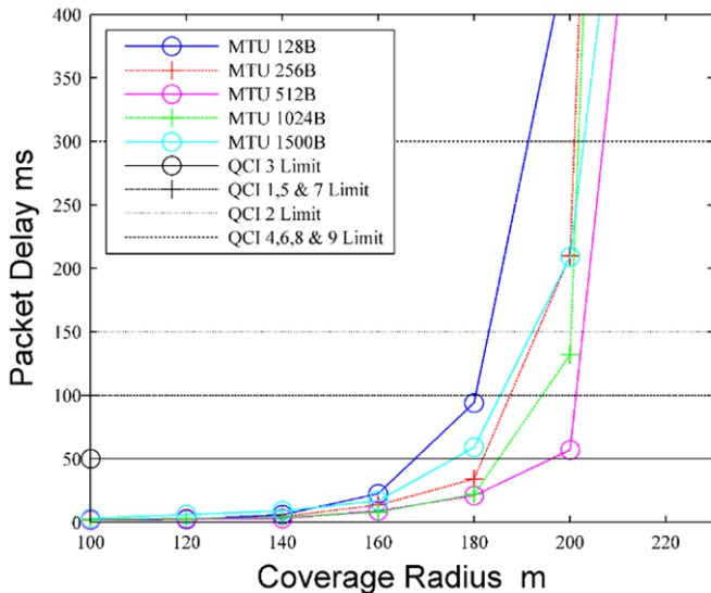
Fig. 4 UK Packet Delay Results
