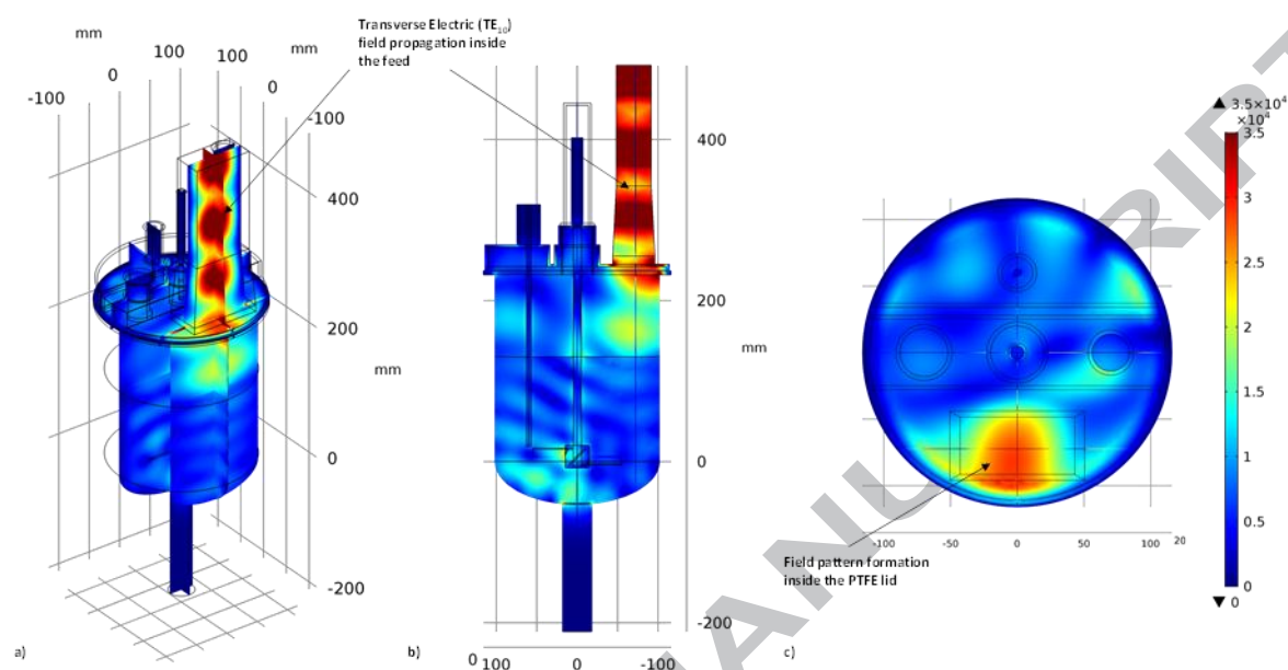
Figure 3: Electric field distribution inside the reactor, a) slice through the width of the waveguide, b) slice through the middle of the depth of the waveguide, c) slice through the top view of the lid side
