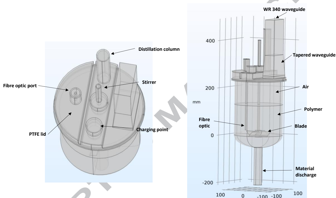
Figure 2: 3-dimensional model of the 5l reactor showing the final lid design, various ports; impeller stirrer, fibre optic thermocouple and microwave in-feed waveguide.
