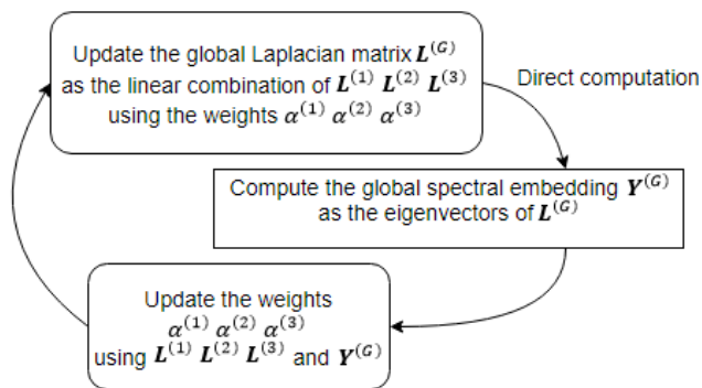
FIGURE 4. Alternate optimization of L^{(G)} and \alpha^{(i)} .
