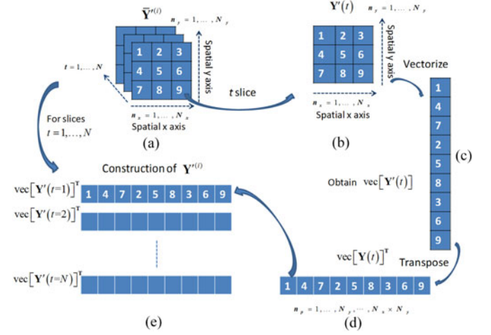
Fig. 5. Illustration of matricizing operation of \bar{Y}^{(i)} .
