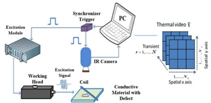
Fig. 3. Inductive thermography diagram.
