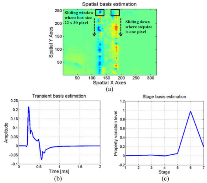
Fig. 10. The decomposition results for gear fatigue test: (a) Spatial basis, (b) transient basis, and (c) stage basis.
