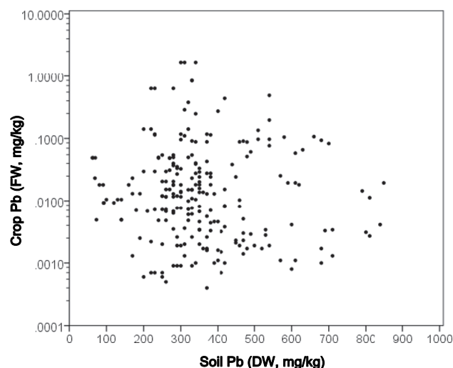
Fig. 2. Association between soil Pb and crop Pb concentrations ( \text{mg/kg} ). (Spearman's r = -0.112 , p = 0.085 ). Note: two soil outliers have been removed for presentation purposes (one at 1200 \text{ mg/kg} and one at 6300 \text{ mg/kg} ).
