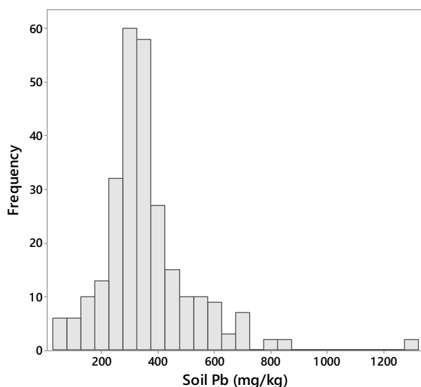
Fig. 1. Pseudo-total Pb concentration in the soils ( \text{mg/kg} , n = 279 ), excluding one outlier ( 6300 \text{ mg/kg} ).
