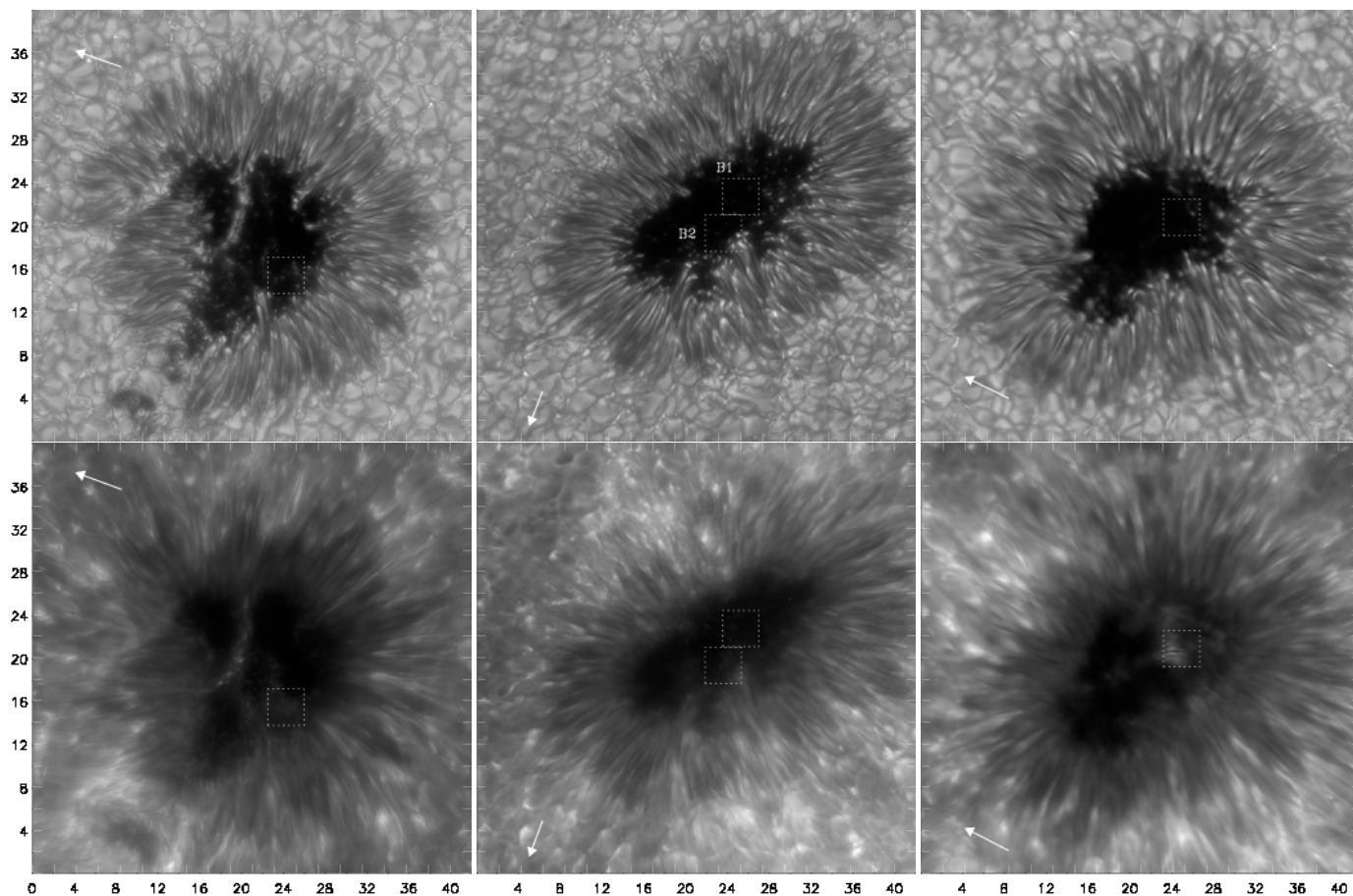
Fig. 1. Three sunspots analysed in this work. Top row: wideband images and bottom row: Ca II H core filter images. The arrows point towards the solar disk centre. The field of view is 42 \times 42'' with tickmarks at 2'' intervals. The boxes delimit the regions of interest shown in Fig. 2.
