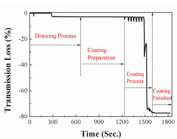
FIGURE 3: Transmission loss of OFM during drawing and coating processes.
