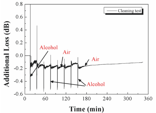
FIGURE 7: Repeatability of the response of an OMF sensor with a diameter of 5 μm when immersed in alcohol eight times.
