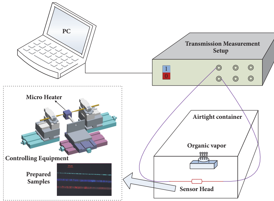
FIGURE 2: Experimental setup of coated OMF sensor.
