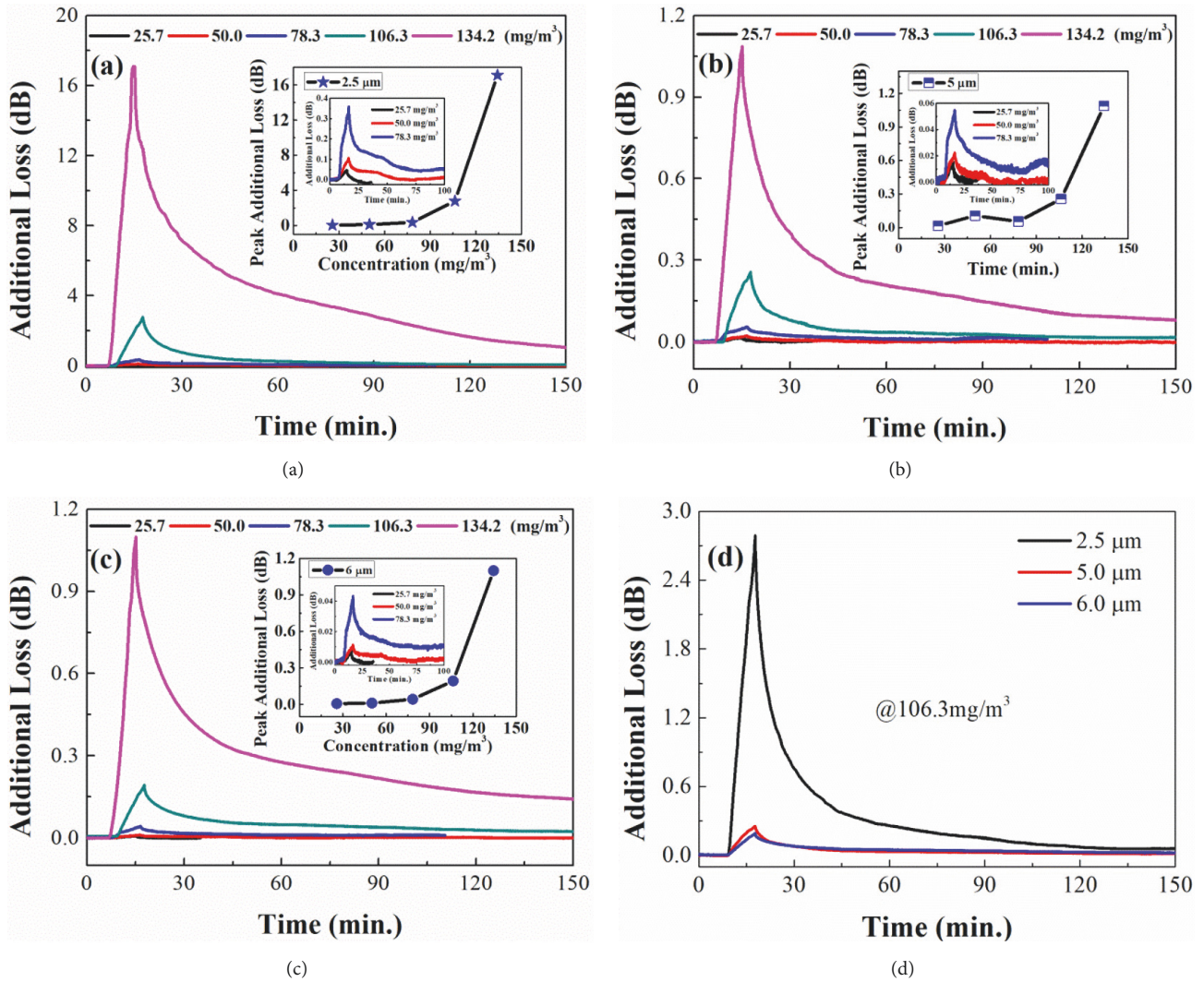
FIGURE 6: Responses of coated OMF sensor at different concentrations of AMCs from 25.7 to 134.2 mg/m 3 with three different diameters of (a) 2.5 μm, (b) 5 μm, and (c) 6 μm and (d) response results of OMF sensor obtained at 106.3 mg/m 3 with three different diameters.
