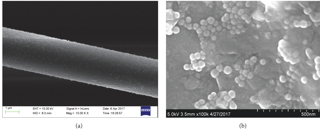
FIGURE 4: Surface morphology of the OMF with HSNs (a) at 15kv and 10k \times and (b) at 5kv and 100k \times .
