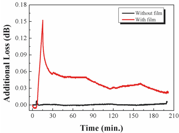
FIGURE 5: Sensitivity and recovery responses of coated and naked OMF sensors (diameter, \sim 5 \mu\text{m} ) to AMCs at a concentration of 106.3 \text{ mg/m}^3 .
