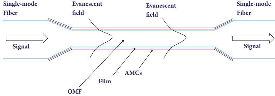
FIGURE 1: Principle of molecular contaminants adhered on microfibre with HSNs film.
