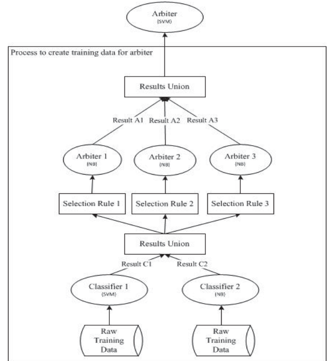
Fig. 2. Process for making training data for arbiter.
