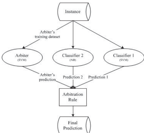
Fig. 3. Process for final prediction of the testing data of arbiter tree.
