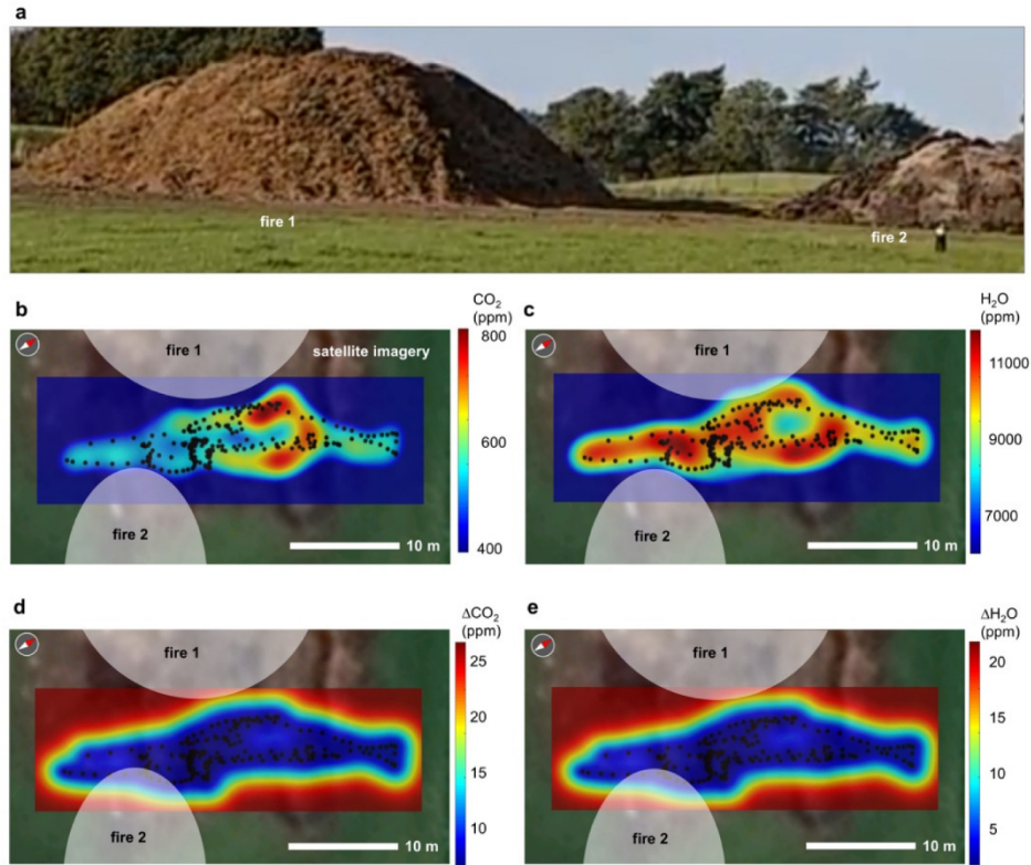
Fig. 3. Mapping atmospheric carbon dioxide and water-vapor distributions. (a) Site image illustrating the two dung-heap fires, between which the UAV was flown. No flames were visible from the fires. (b, c) Concentration maps produced from data recorded for (b) carbon dioxide and (c) water vapor during manual flight between two dung fires. Sampling points are shown in black. (d, e) Corresponding gas concentration uncertainty maps for (d) carbon dioxide and (e) water vapor, obtained from the Gaussian-process fitting. Satellite imagery ©2018 Google, used with permission under Google Terms of Service.
