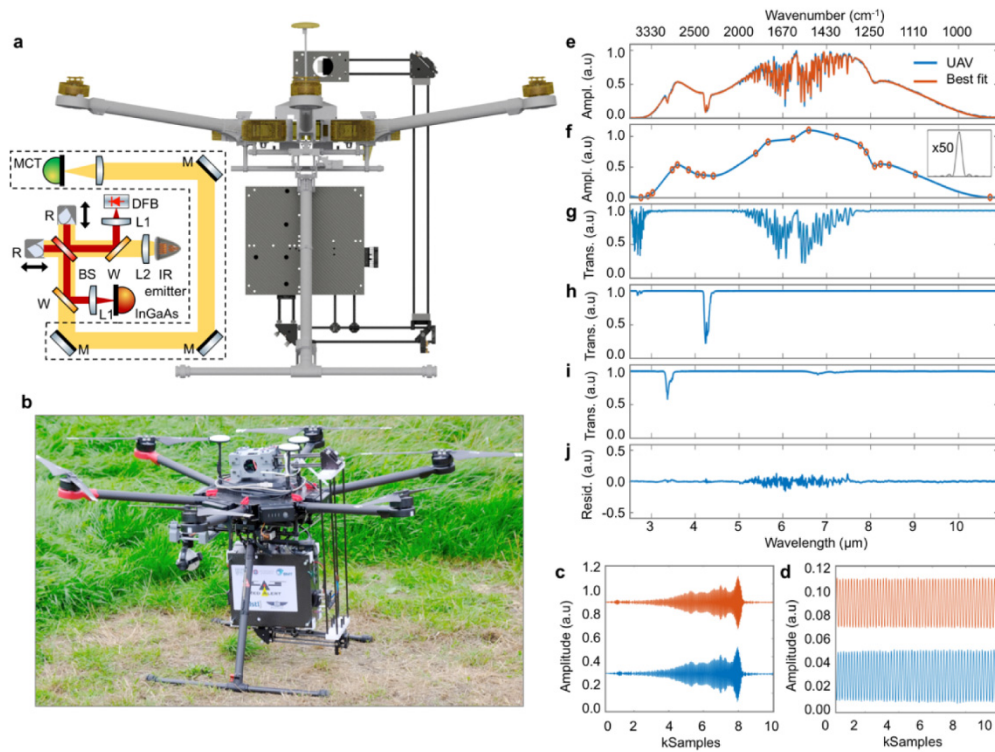
Fig. 1. Optical configuration and in-flight performance data for the UAV-mounted Fourier-transform spectrometer. (a) UAV schematic showing spectrometer suspended underneath, and the C-shaped sensing path (dashed line) of 1 m length. DFB, 1550-nm single-frequency laser diode; L1, aspheric lenses (coated for 1.5 \mu\text{m} ), L2, ZnSe lenses; BS, \text{CaF}_2 beamsplitter; W, Ge windows; R, retroreflectors; M, silver mirrors; InGaAs, InGaAs photodiode; MCT, MCT detector. (b) The assembled system in field trials. (c) Representative mid-infrared and (d) reference laser interference fringes obtained from the UAV before take-off (red), and in-flight (blue). (e) Infrared absorption spectrum obtained in flight (blue) and least squares fit (red). (f) Fitted envelope, which is modelled as a spline curve with the positions of the anchor points (symbols) being unconstrained fitting parameters; inset: fitted \text{sinc}^2(v) instrument function, corresponding to the triangular apodization used. (g–i) Fitted transmittance spectra for water, carbon dioxide and propane. These spectra, obtained during a propane sensing flight, show a background \text{CO}_2 level of 400 ppm and concentrations for water of 1.16% and for propane of 362 ppm. (j) The fitting residual between the two spectra in (e), presented on the same scale. Insufficient instrument resolution to resolve the dense and saturated line structure of water in the 5 – 7- \mu\text{m} region leads to the remaining fitting uncertainty here.
