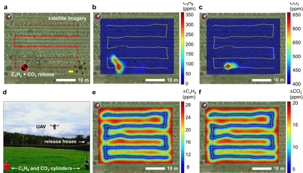
Fig. 2. Localisation of point sources of gas emissions. (a) Flight plan and (d) site image, showing the location of the propane and carbon dioxide gas sources. (b, c) Gas concentration and (e, f) accompanying uncertainty maps prepared by Bayesian interpolation of the recorded concentration data for propane and for carbon dioxide. The maximum likelihood locations of the carbon dioxide and propane sources are denoted, respectively, by the green and red crosses, with the error bars being the spatial sampling resolution. Satellite imagery ©2018 Google, used with permission under Google Terms of Service.
