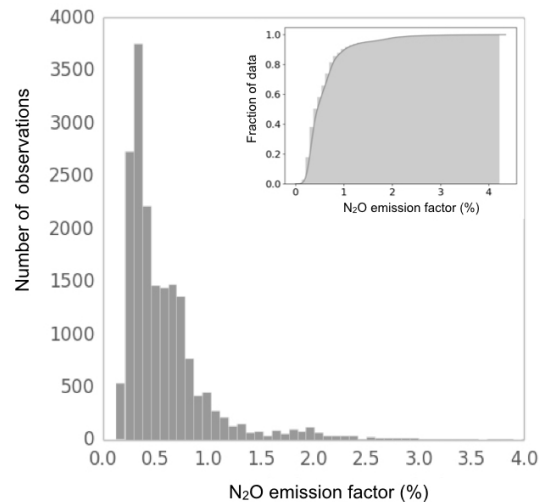
Figure 5. The distribution and cumulative distribution (small graph) of simulated N 2 O EFs
